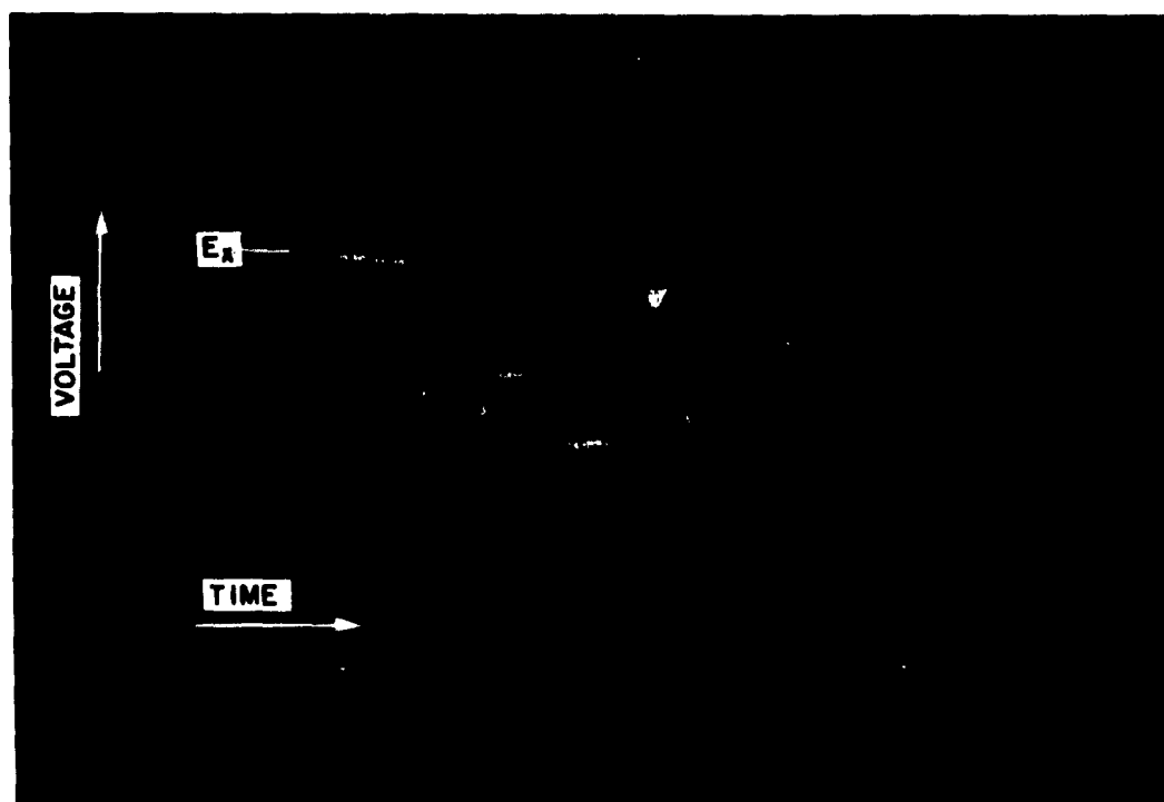
Figure 6. (b) Oscillogram of plate impact test with suspected spalling. Time marks at 0.1 \mu sec intervals.
