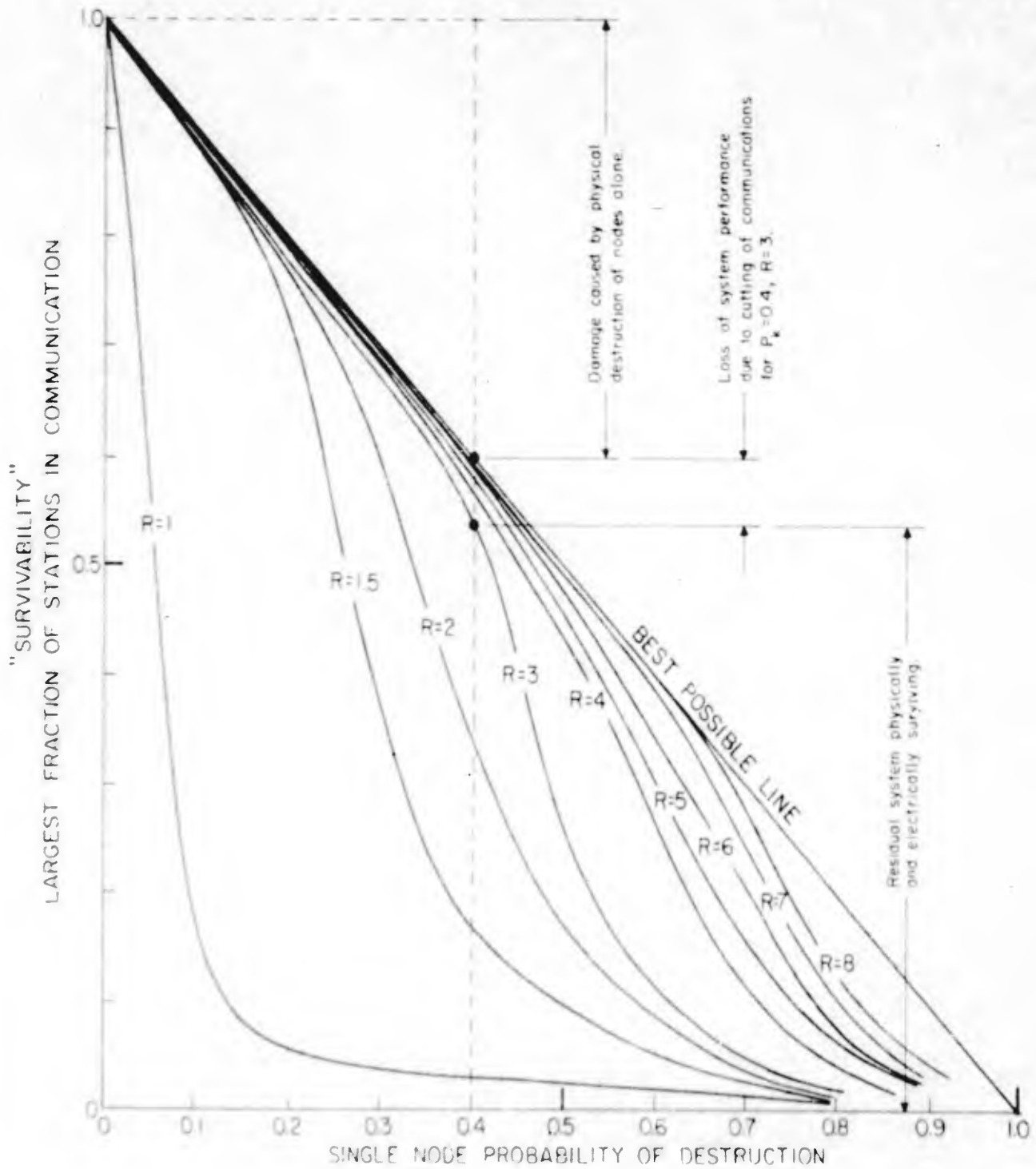
FIG. 4 - Perfect Switching in a Distributed Network - Sensitivity to Node Destruction, 100% of Links Operative
