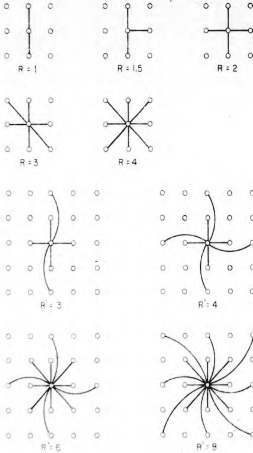
FIG. 2 - Definition of Redundancy Level
