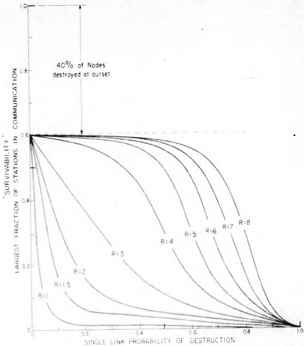
FIG 6 - Perfect Switching in a Distributed Network - Sensitivity to Link Destruction After 40% Nodes Are Destroyed.
