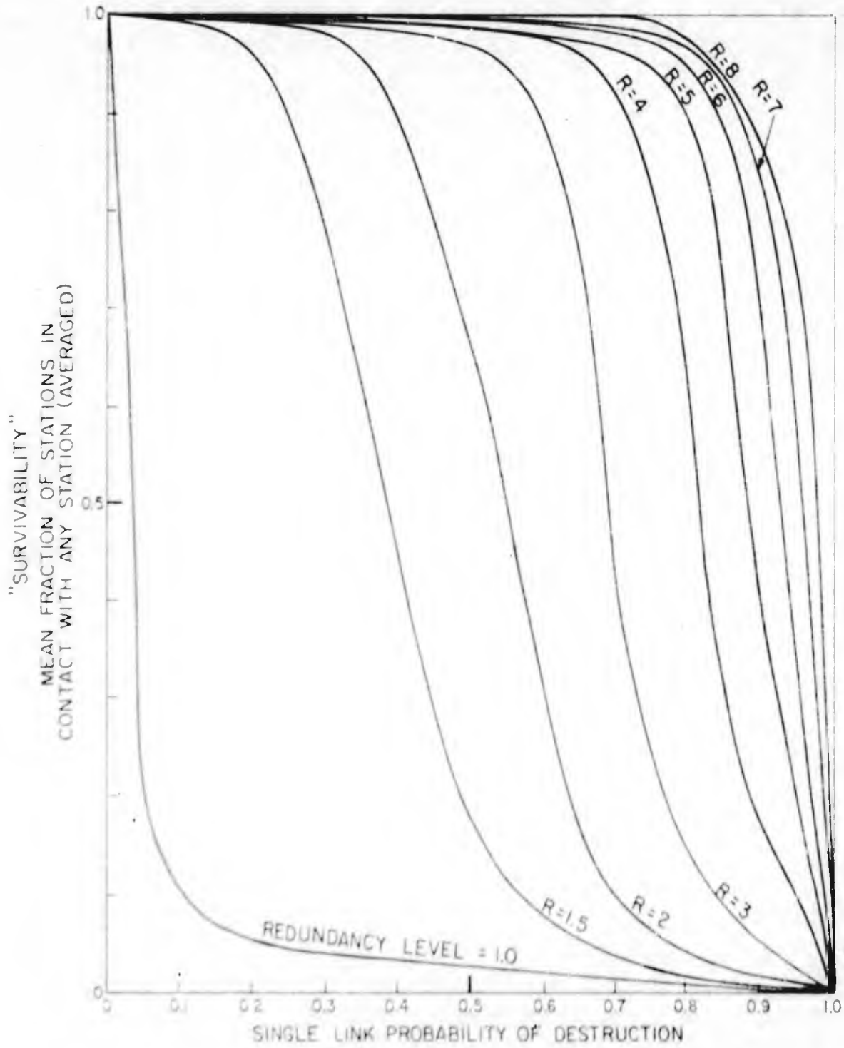
FIG. 5 - Perfect Switching in a Distributed Network - Sensitivity to Link Destruction, 100% of Nodes Operative
