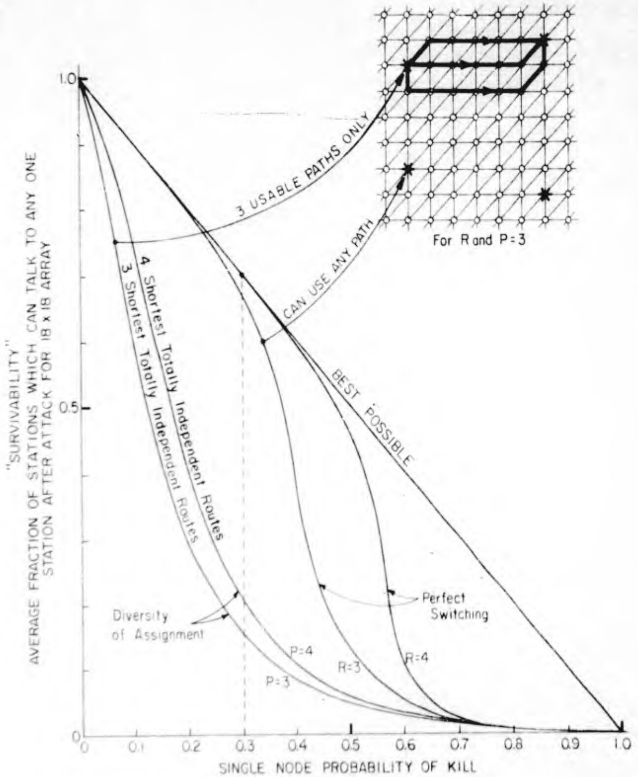
FIG 8 -- Diversity of Assignment vs Perfect Switching in a Distributed Network.
