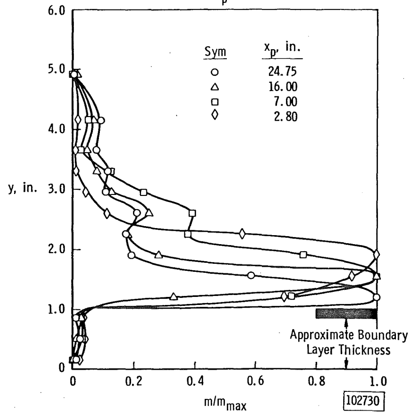
a. Variation of Nozzle Position; d_i = 0.15 in., p_{o_i} / p_\infty = 60 Fig. 4 Particle Distribution on Tunnel Centerline at M_\infty = 3
