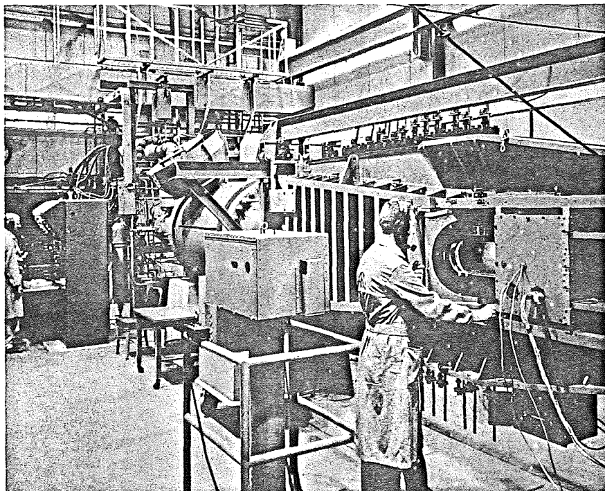
Fig. 1 Tunnel D
