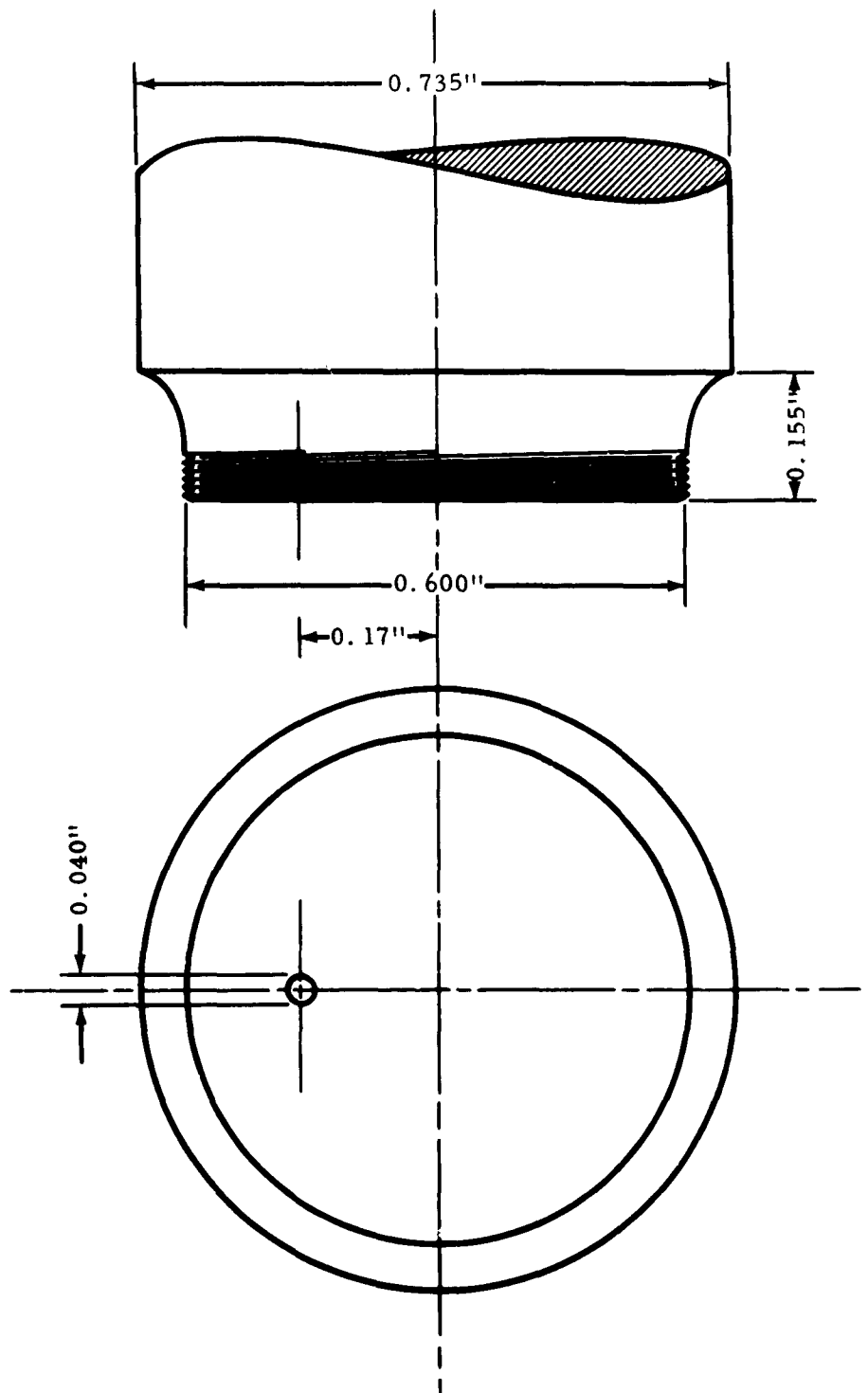
FIGURE 3 A SKETCH OF AN ALTEC LANSING PIN HOLE MICROPHONE
