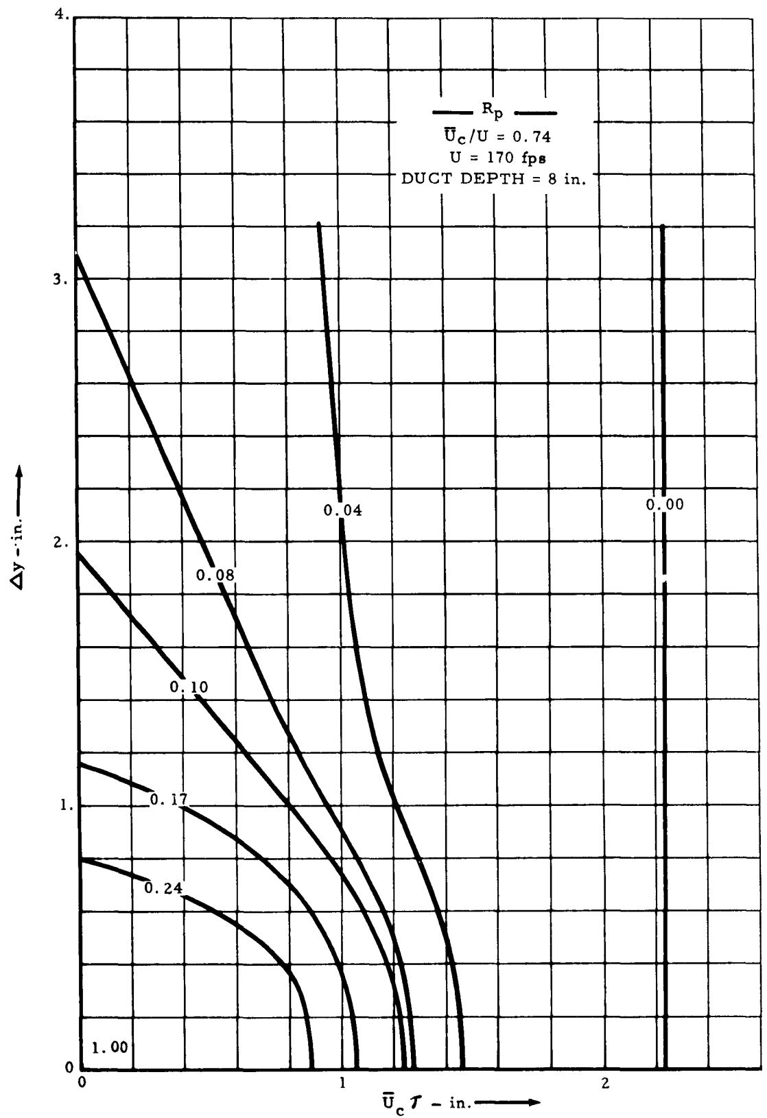
FIGURE 18 LINES OF CONSTANT LATERAL CORRELATION: WALL PRESSURE FLUCTUATIONS
