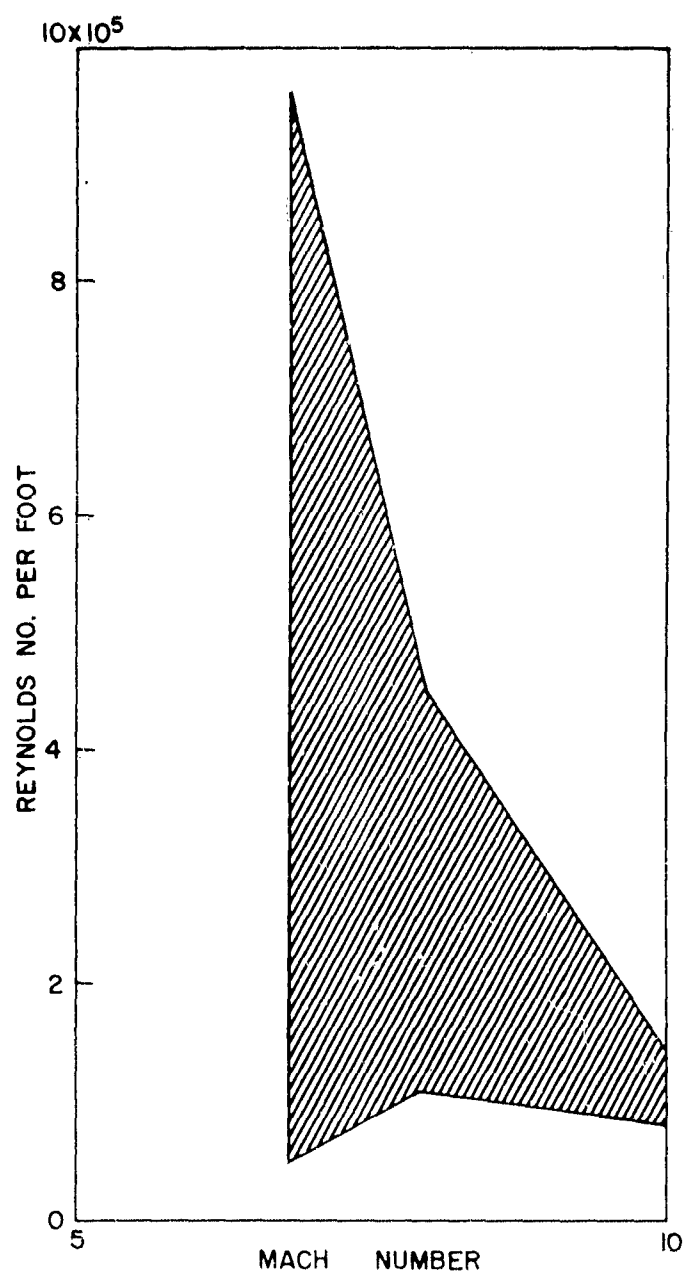
FIG. 26 REYNOLDS NUMBER CAPABILITY
