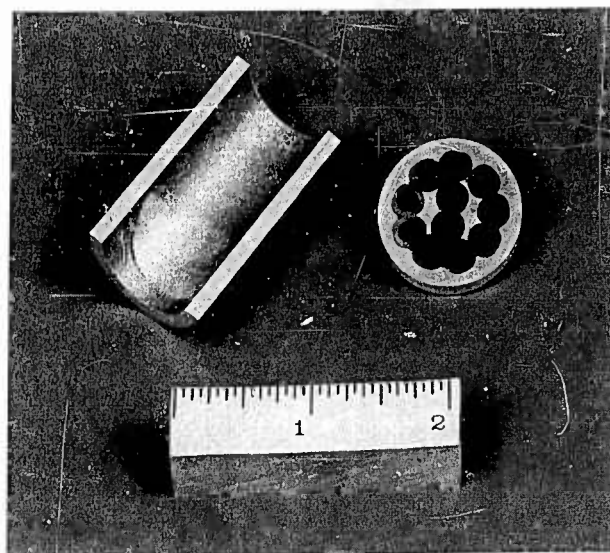
Fig. 20 Explosively bonded, cylindrical aluminum components
