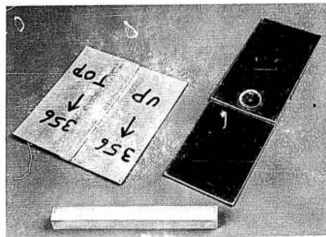
Fig. 6 Explosively welded lap joints in 1/16 -in. aluminum alloy 2024-T3. Left: seam weld; right: spot weld
