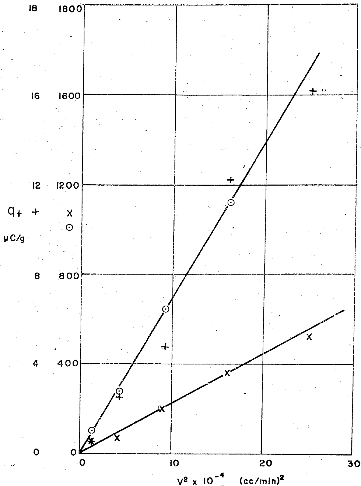
Figure 14. Positive Charge per Gram Positive Deposit, q_+ , as a Function of Square of Flow Rate, v . ○ MgO, X NH 4 Cl, + Polyvinyl Chloride.
