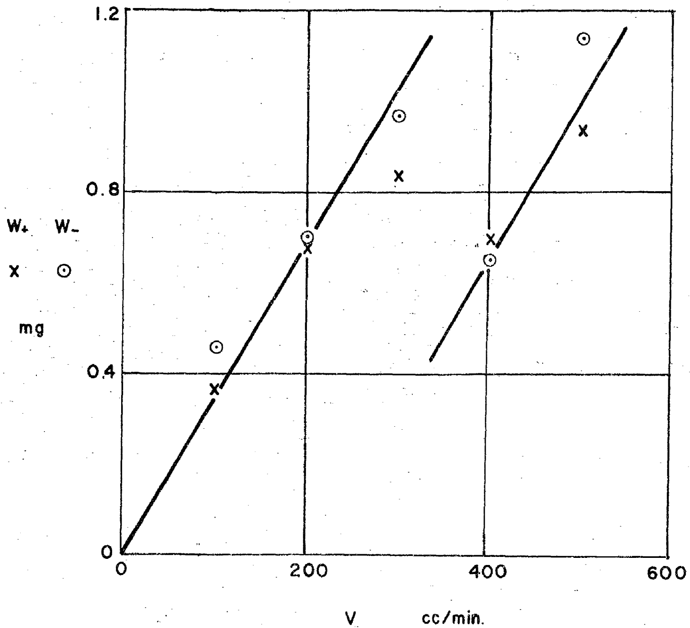
Figure 8. Positive Deposits w_+ (x) and Negative Deposit w_- (o) in One Minute for MgO as Functions of Flow Rate v .
