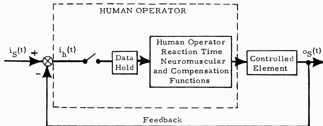
Figure 11. Simple sampled-data model (after Bekey, 1962, p. 44)
