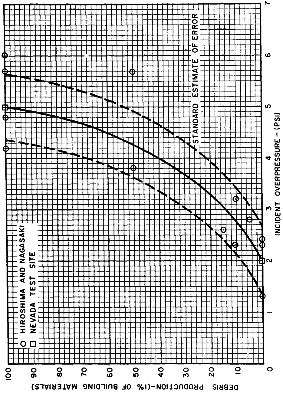
Figure 19. Debris Production vs. Overpressure; Wood Frame Buildings
