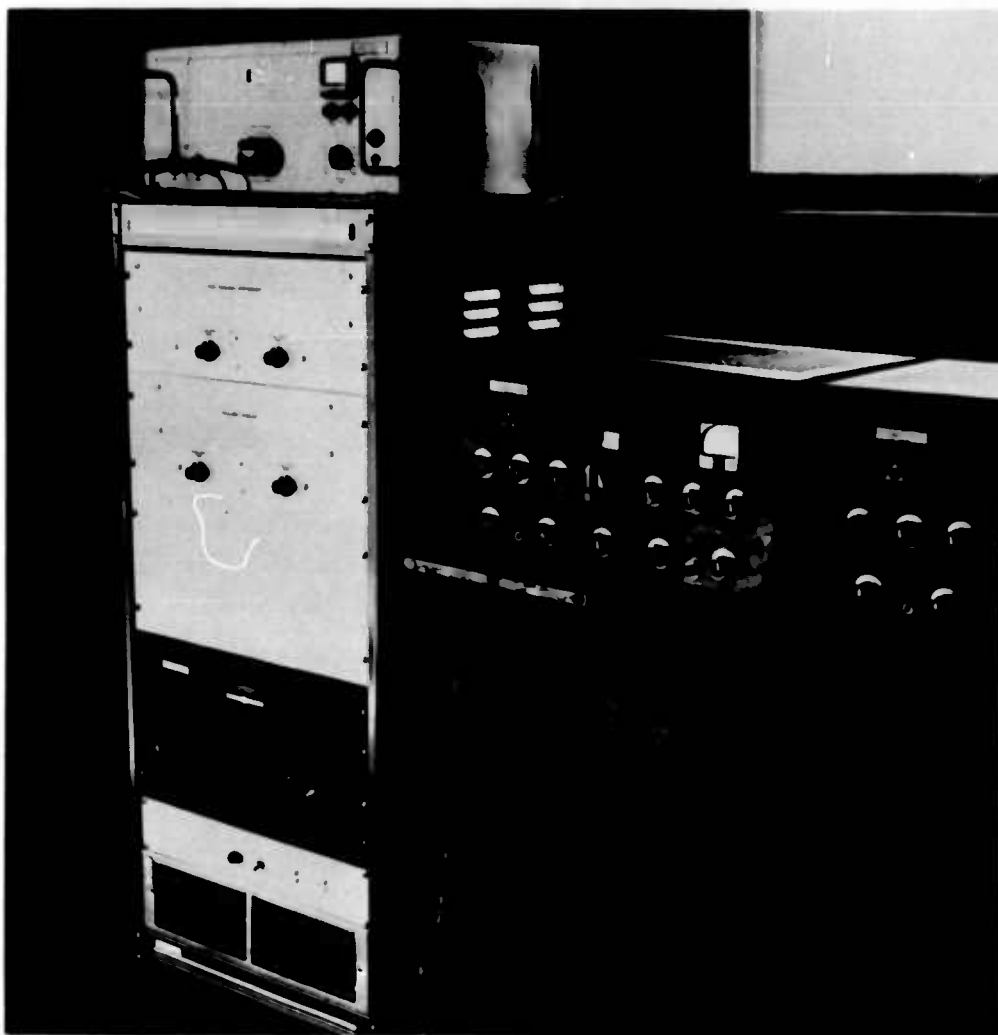
FIG. 7. INTERIOR OF TRANSMITTER BUILDING SHOWING FREQUENCY STANDARD, FREQUENCY SYNTHESIZER AND TRANSMITTER.
