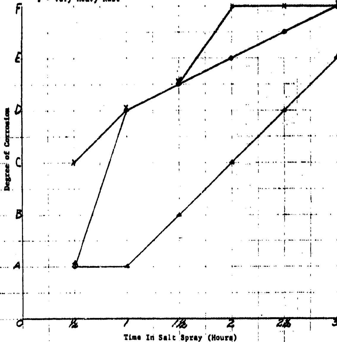
FIGURE 2. EFFECT OF ULTRASONIC CLEANING IN WATER AND WATER PLUS DETERGENTS ON MANGANESE PHOSPHATE PANELS
