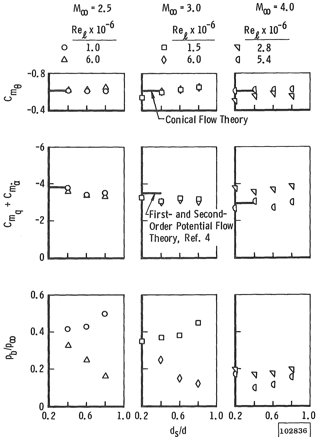
Fig. 6 Slope of the Pitching-Moment Curve, Damping-in-Pitch Derivatives, and Base Pressure Ratio versus Sting Diameter Ratio for \ell_s/d = 3
