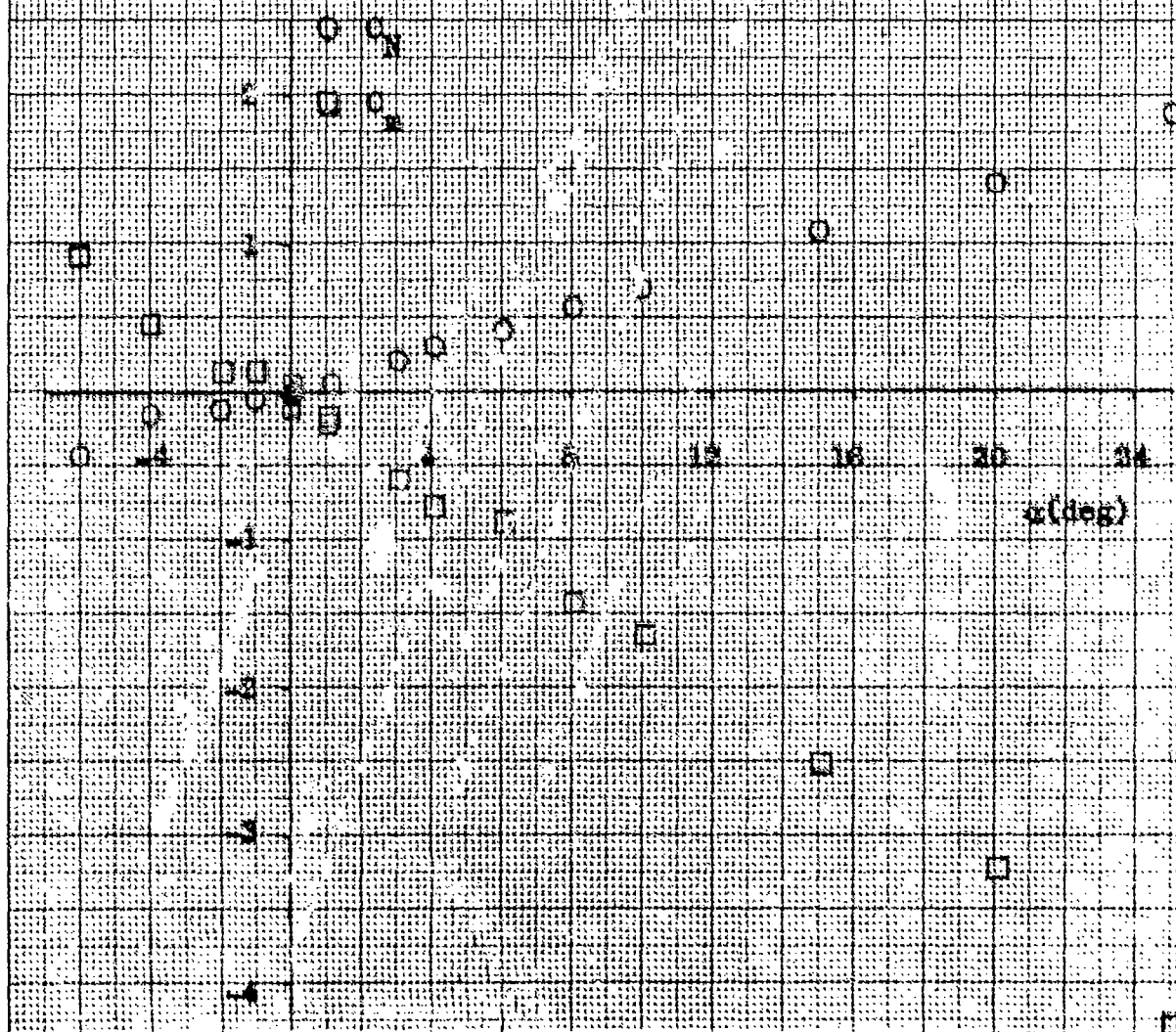
FIG. 35 NORMAL FORCE COEFFICIENT AND PITCHING MOMENT COEFFICIENT VERSUS ANGLE OF ATTACK FOR CONFIGURATION SLT 1 AT MACH NUMBER 0.23
