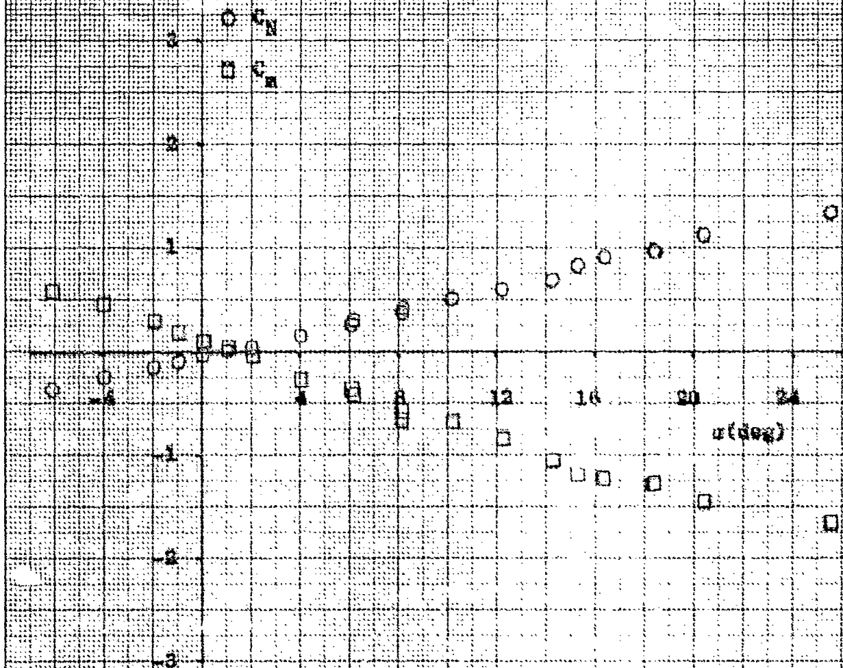
FIG. 27 NORMAL FORCE COEFFICIENT AND PITCHING MOMENT COEFFICIENT VERSUS ANGLE OF ATTACK FOR CONFIGURATION B11 AT MACH NUMBER 0.72
