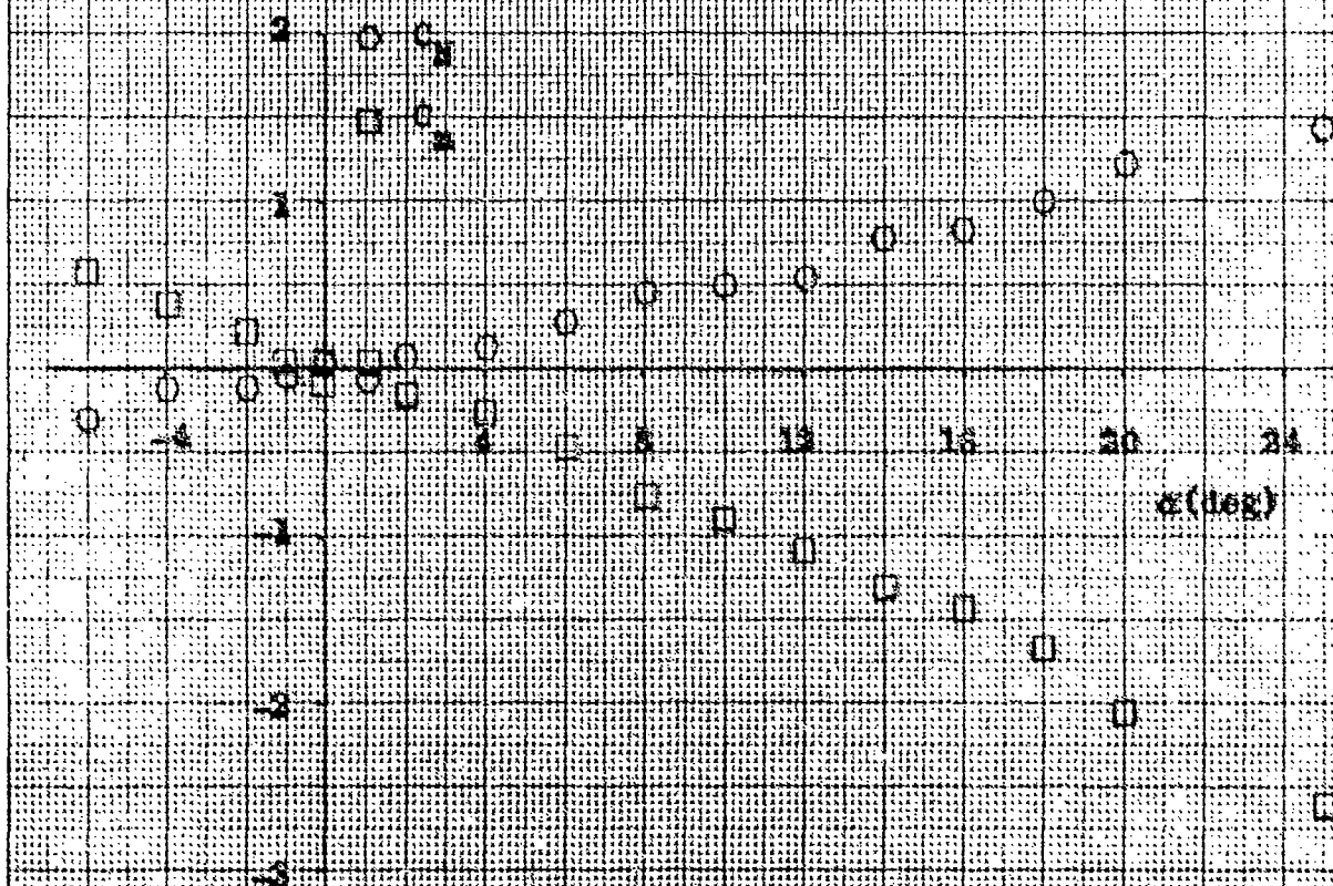
FIG. 34 NORMAL FORCE COEFFICIENT AND PITCHING MOMENT COEFFICIENT VERSUS ANGLE OF ATTACK FOR CONFIGURATION HL-10 AT MACH NUMBER 0.23
