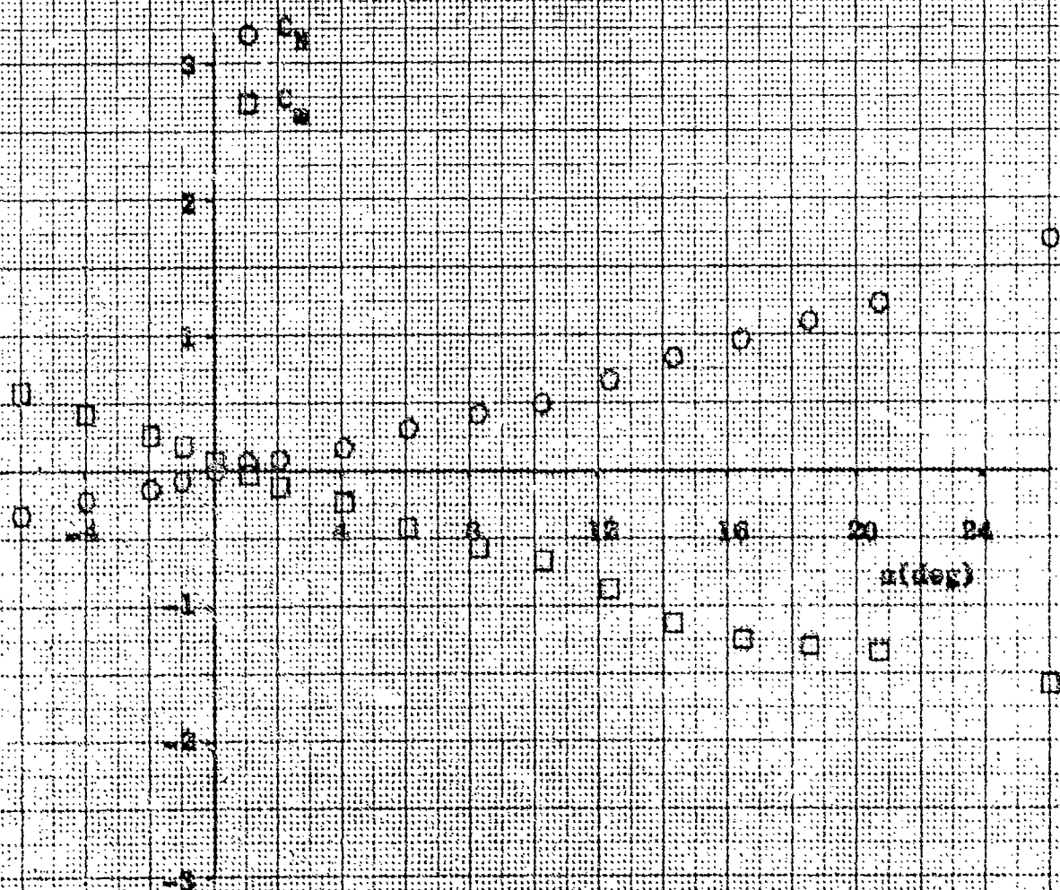
FIG. 30 NORMAL FORCE COEFFICIENT AND PITCHING MOMENT COEFFICIENT VERSUS ANGLE OF ATTACK FOR CONFIGURATION B1-7 AT MACH NUMBER 0.85
