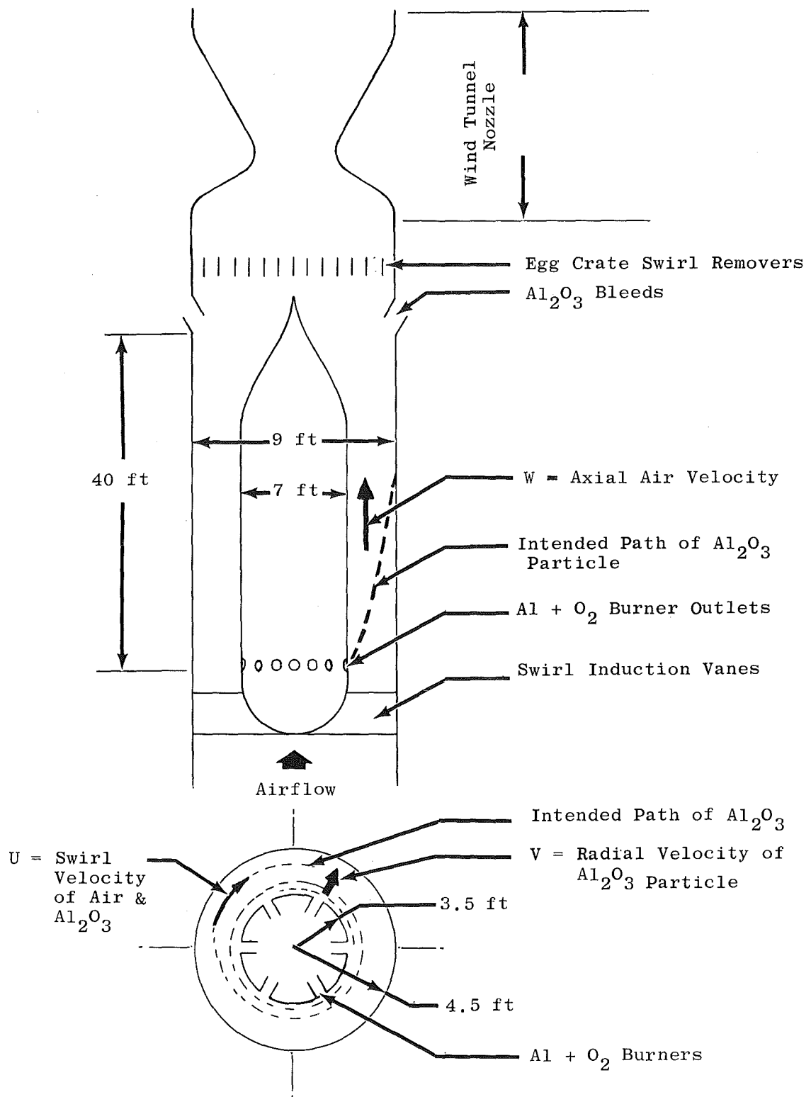
Fig. 3 Possible Configuration for Centrifugal Separation of Al_2O_3 from Air
