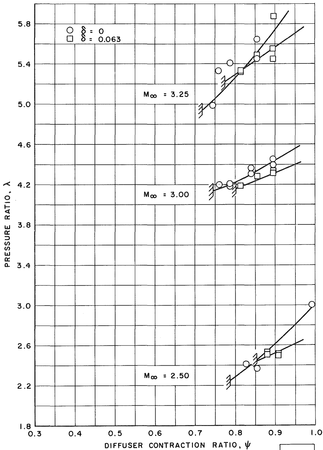
Fig. 14 Effect of Test Section-Diffuser Gap on the "A" Family Starting and Running Performance at M = 2.50, 3.00, \text{ and } 3.25 ; \theta_w = -30^\circ
