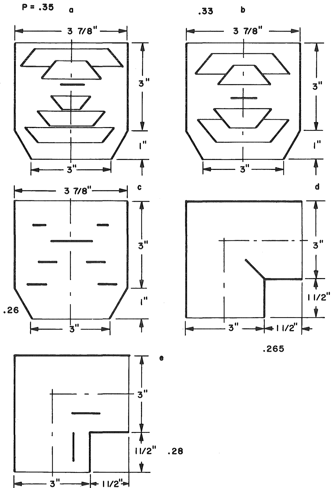
Fig. 13 Baffle Models
