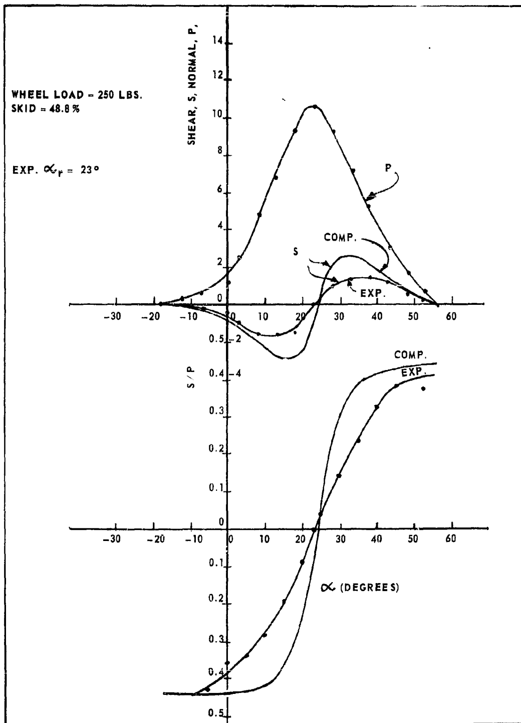
FIG. 33 SOIL STRESSES, SHEAR (S) AND NORMAL (P) UNDER A BRAKED, RIGID WHEEL IN SAND.
