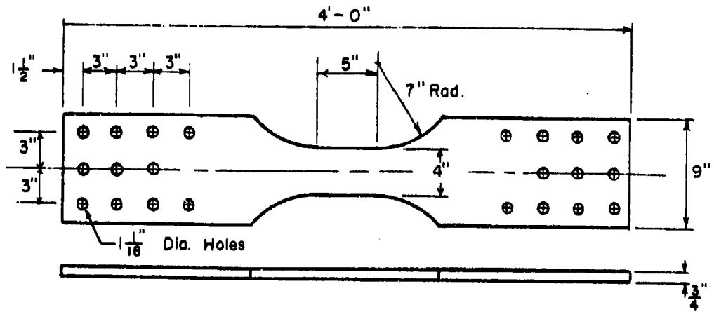
(a) Plain Plate
