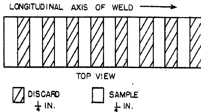
FIG 6.3 SECTIONING PLAN FOR METALLOGRAPHIC SAMPLES OF BUTT WELDED HY-80 STEEL.
