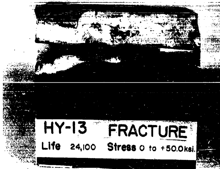
b) FAILURE INITIATED IN WELD.
