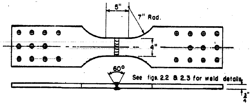
(b) Transverse Butt Weld
