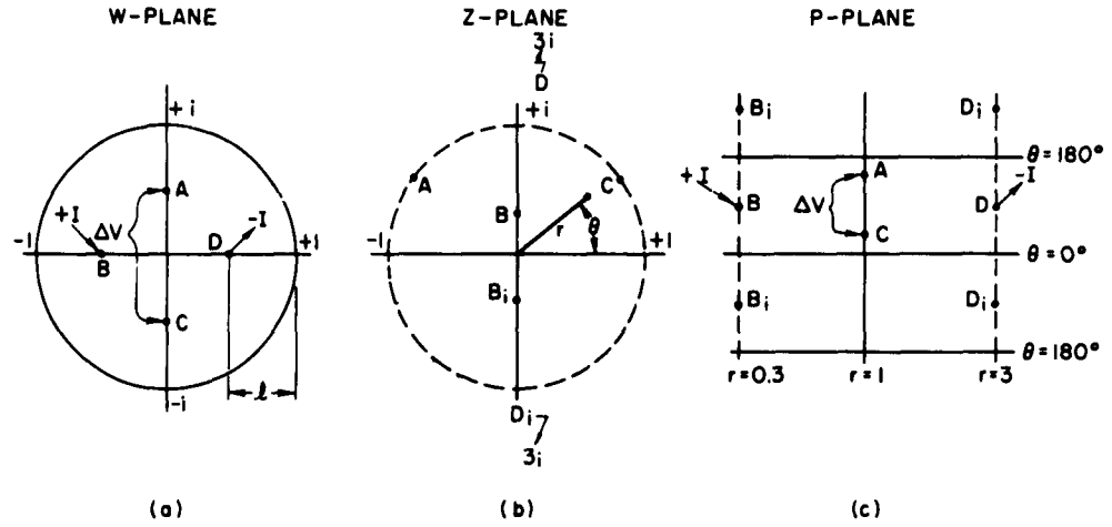
FIG. 99. HALL COEFFICIENT MEASUREMENT ON A CIRCULAR SAMPLE . WITH CONTACTS MUTUALLY 90^\circ APART AND DISPLACED A DISTANCE \ell FROM THE PERIPHERY. Magnetic field is perpendicular to page.
