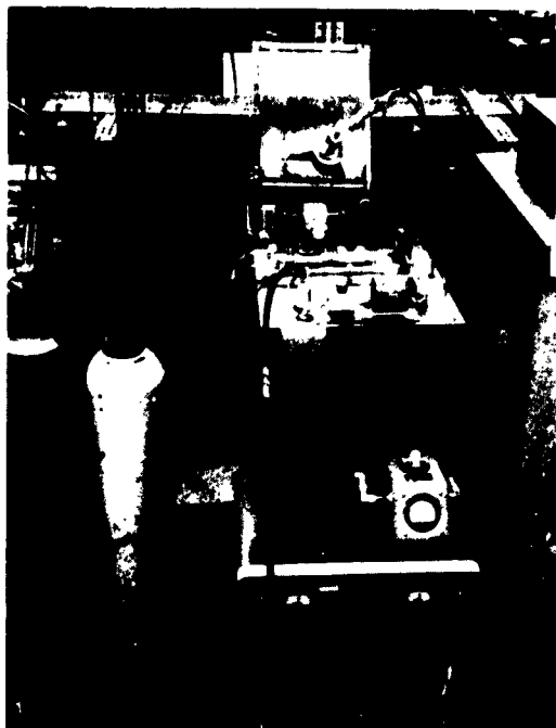
FIG. 8. PIPER. WITH 140 Mc CAVITY IN PLACE. Also visible is an 8 mm interferometer used for density measurements.
