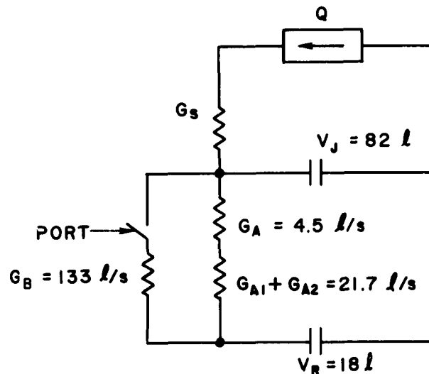
FIG. 33. SPECIAL CASE FOR CALIBRATING LEAK VALVE.
