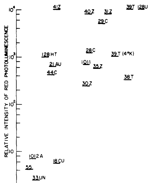
FIG. 87. RELATIVE RED PHOTOLUMINESCENCE OF DIFFERENT GaP CRYSTALS.
