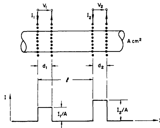
FIG. 46. PARALLEL PLANE PAIRS OF GRIDS IMMERSED INTO A PLASMA COLUMN AND BELOW TOTAL CURRENT DENSITY I = j + \epsilon_0 \frac{\partial E}{\partial t} AS A FUNCTION OF DISTANCE.
