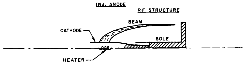
FIG. 34. VTM GEOMETRY.
