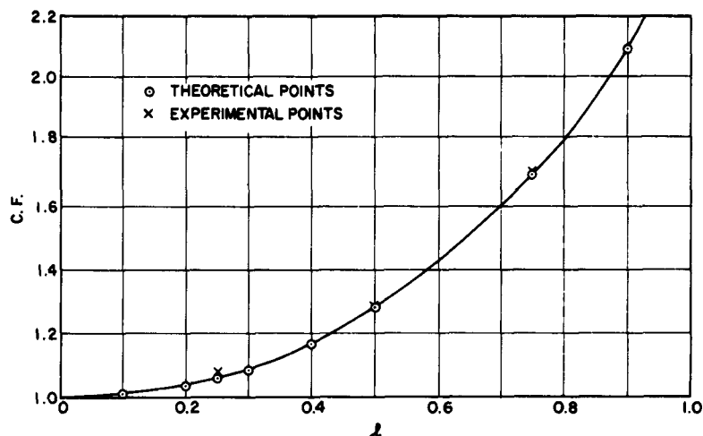
FIG. 98. CORRECTION FACTOR FOR THE RESISTIVITY MEASUREMENT ON A CIRCULAR SAMPLE WITH CONTACTS MUTUALLY 90^\circ APART AND DISPLACED A DISTANCE \ell FROM THE PERIPHERY.
