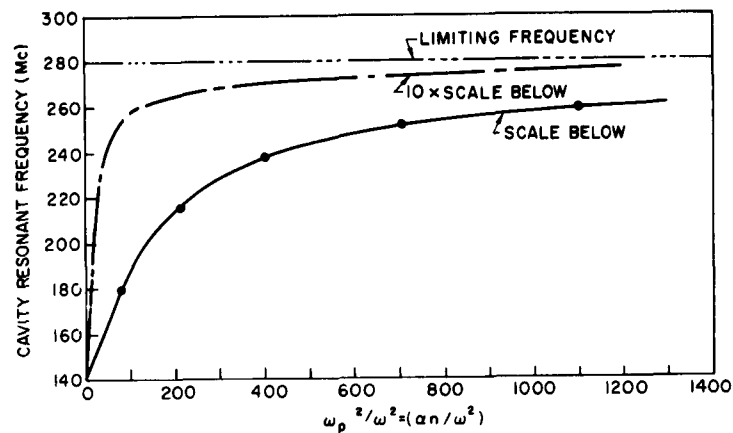
FIG. 10. DEPENDENCE OF CAVITY RESONANT FREQUENCY ON PLASMA DENSITY.
