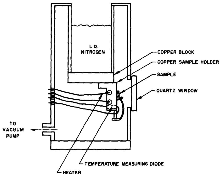
FIG. 106. DEWAR CROSS-SECTION.
