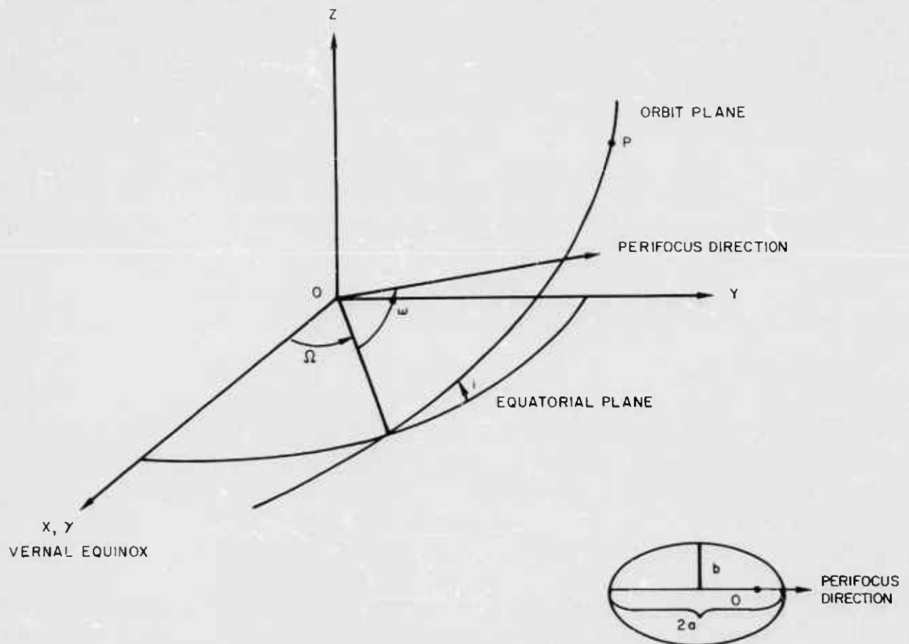
Figure 4. Orbital Elements
