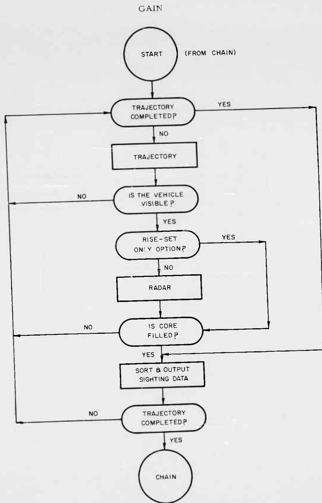
Figure 14. Flow Chart of GAIN Link
