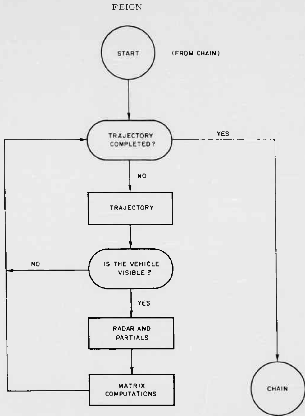
Figure 15. Flow Chart of FEIGN Link
