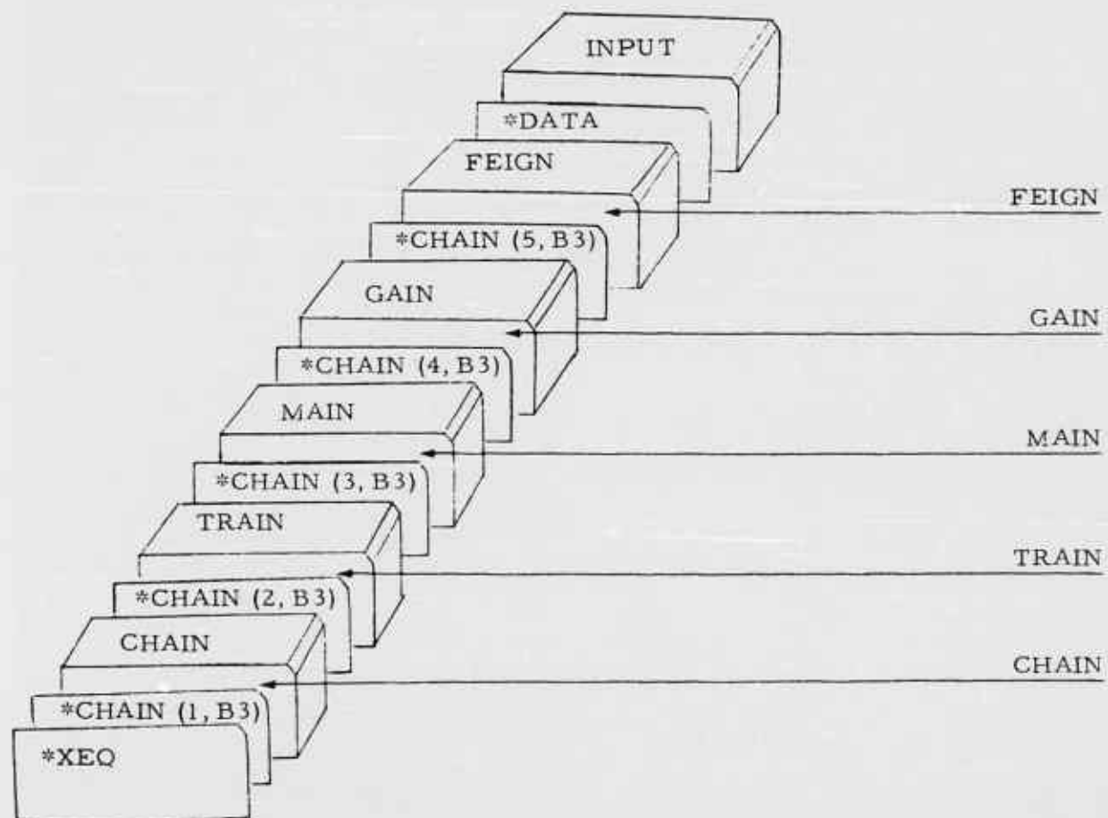
Figure 17. Running from Cards — Complete Deck
