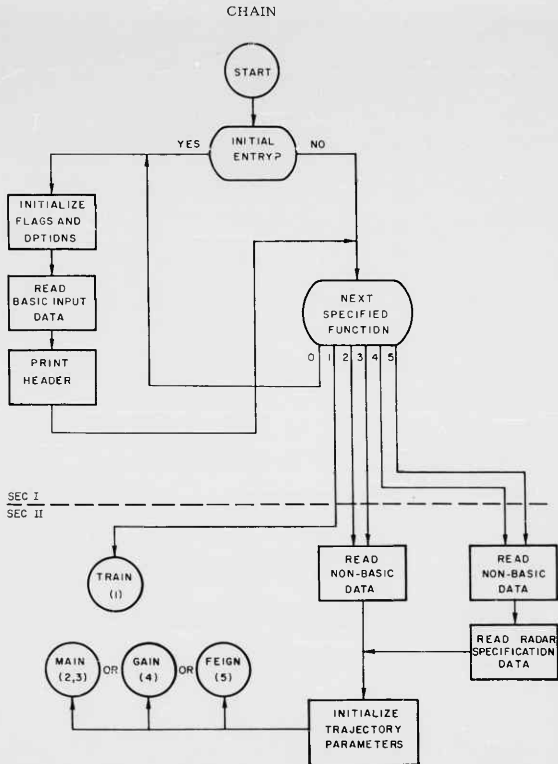
Figure 11. Flow Chart of CHAIN Link
