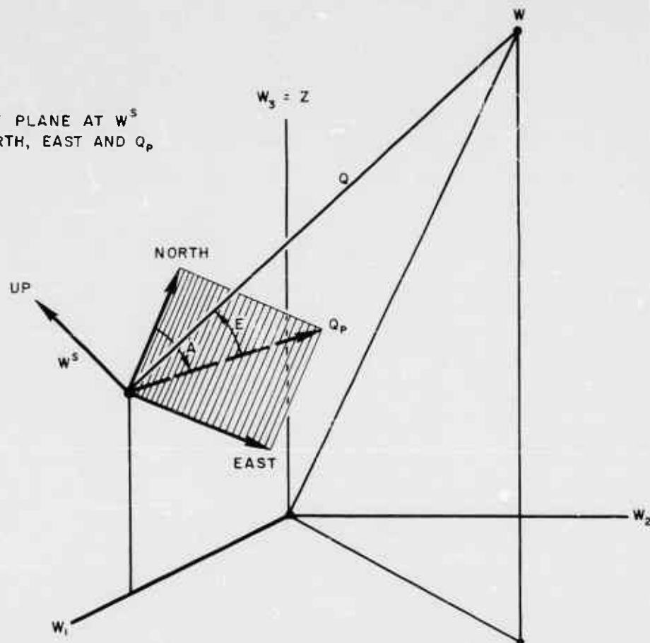
Figure 7. Azimuth and Elevation in Station Coordinate System
