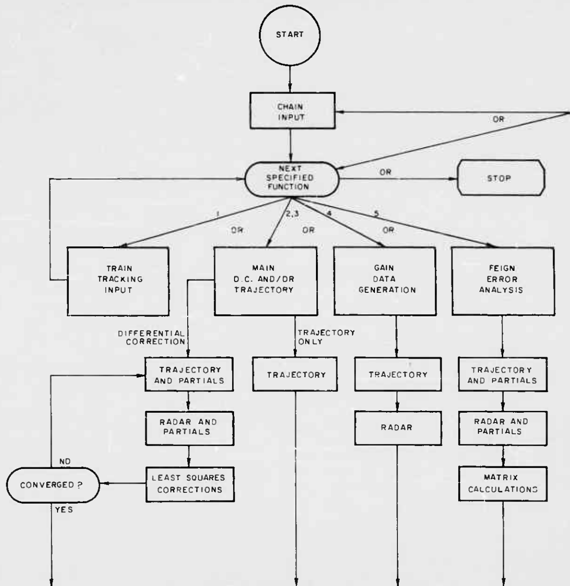
Figure 10. General Flow Chart for TRACE
