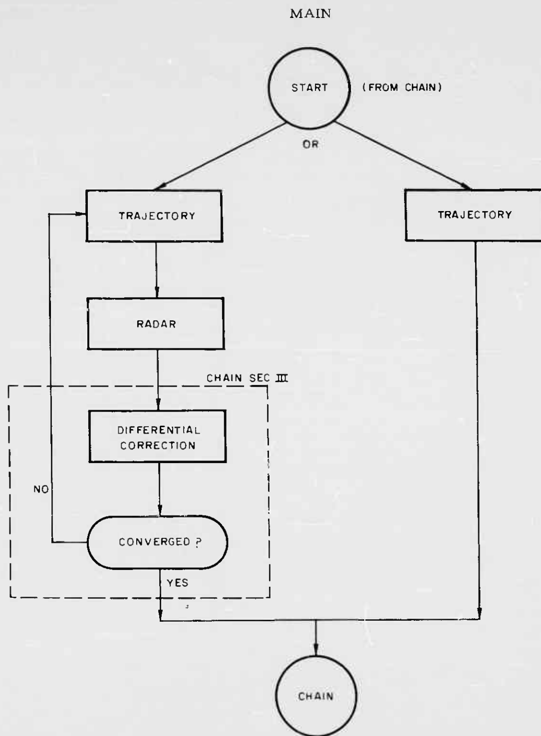
Figure 13. Flow Chart of MAIN Link
