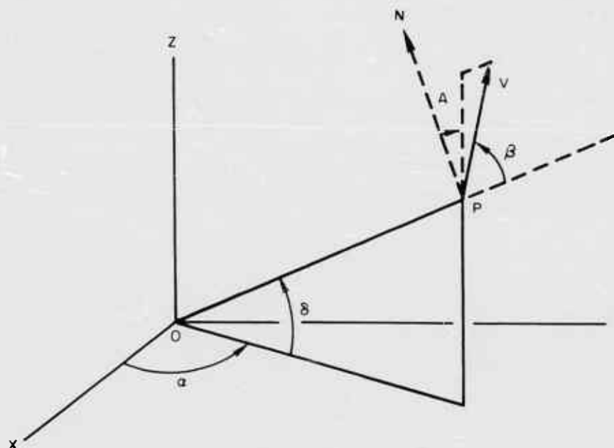
Figure 3. Spherical Coordinates
