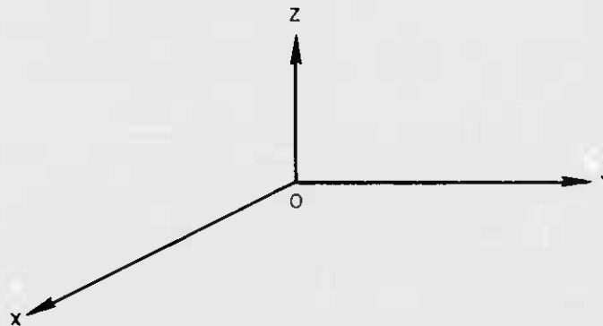
Figure 2. Earth-Centered Coordinate System
