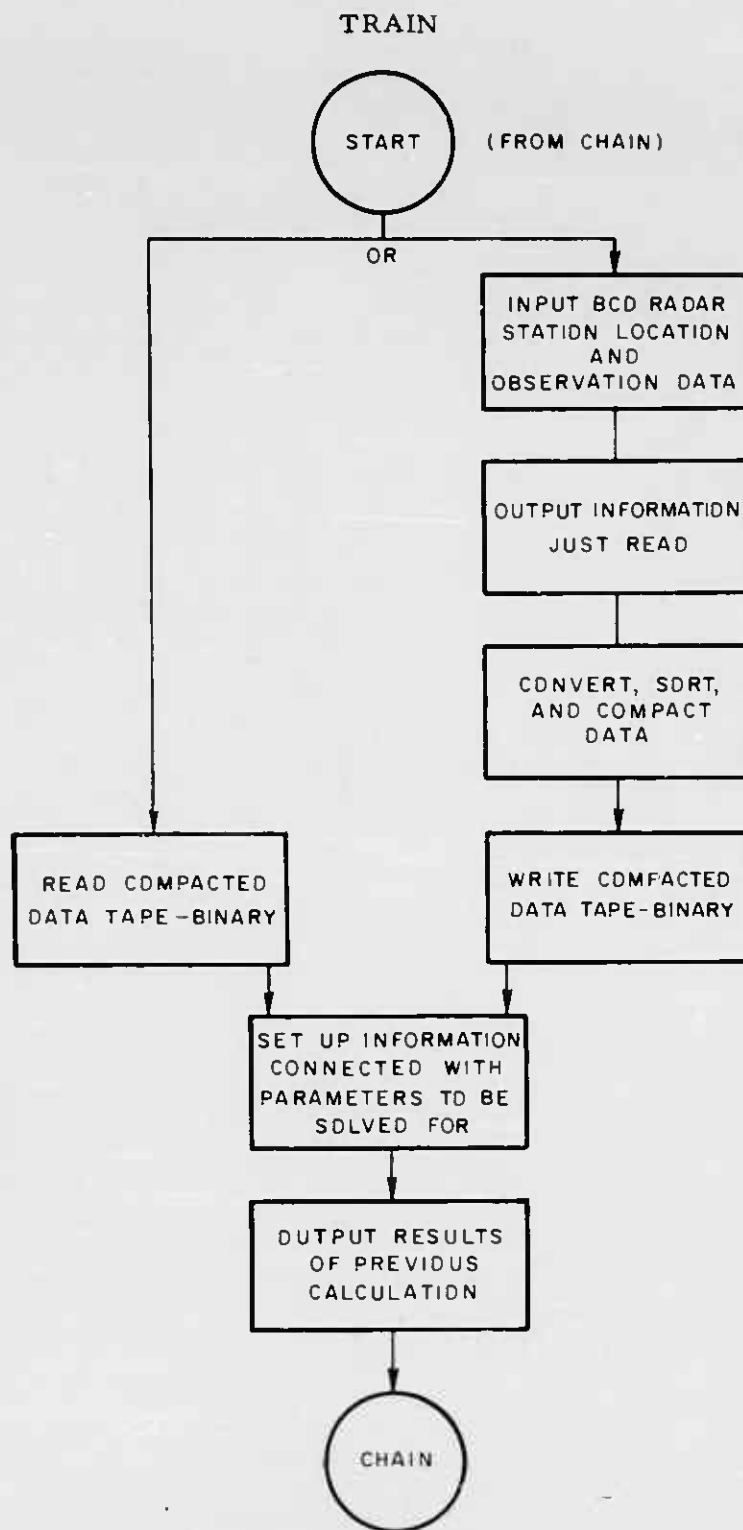
Figure 12. Flow Chart of TRAIN Link
