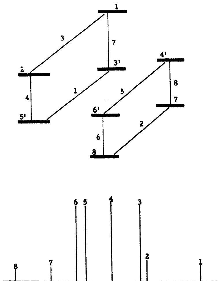
Fig. 5. Schematic energy level diagram and spectrum for the AB part of an ABX spectrum. The illustrated order of energy levels holds for \nu_A > \nu_B , J_{AB} > 0 , and J_{AX} < J_{BX} < 0 . Transitions 1, 2, 3, and 4 are A transitions; 5, 6, 7, and 8 are B transitions.
