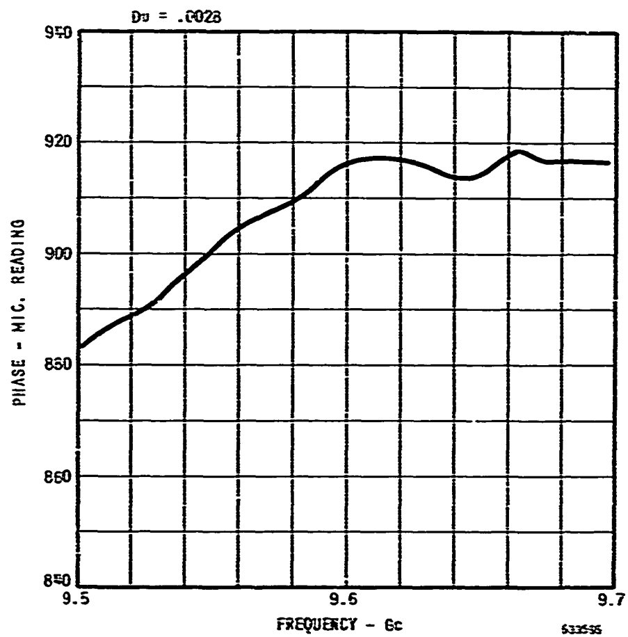
FIGURE 37 PHASE VS FREQUENCY QK5:243/1244 CHAIN #3 (uncorrected)
