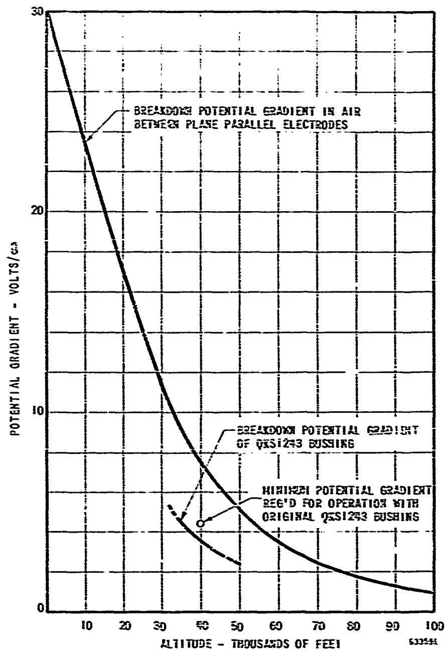
FIGURE 17 HIGH VOLTAGE BUSHING VOLTAGE BREAKDOWN
