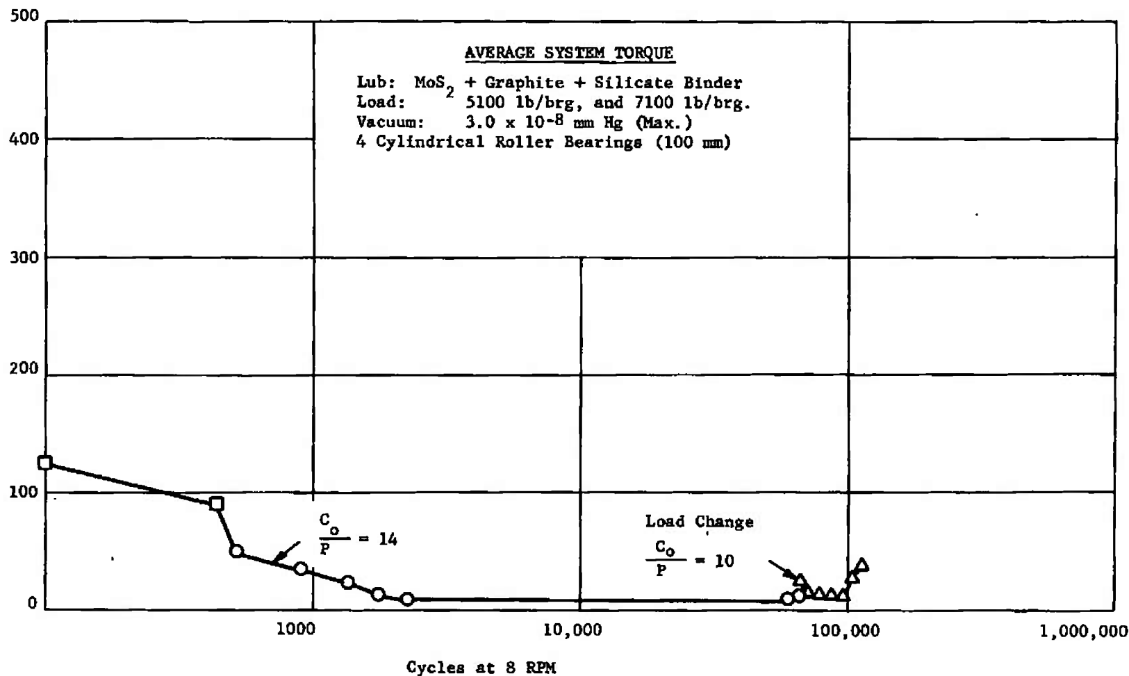
Fig. 41 Average System Torque Curves.
