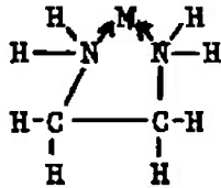
Bidentate Ligand
