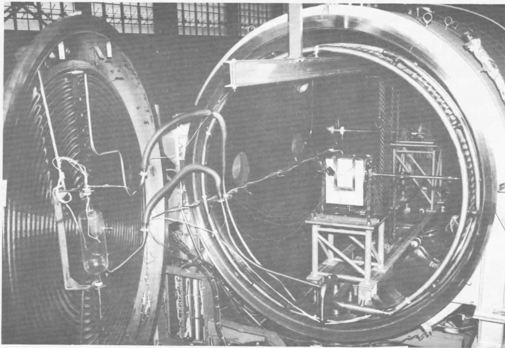
Fig. 29 7 Ft. Aerospace Chamber with Bearing Tester in Foreground and Four Square Gear Tester in Background
