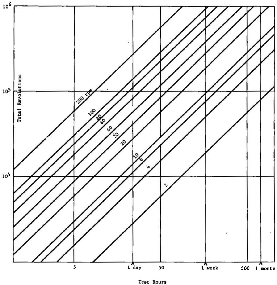
Fig. 7 Total Revolutions versus Test Time at Various Speeds
