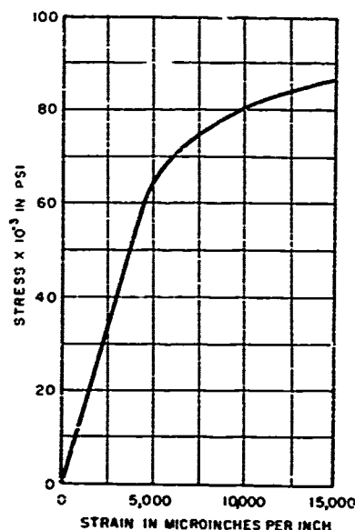
Figure 1 - Typical Stress-Strain Curve for 7075-T6 Aluminum Alloy
