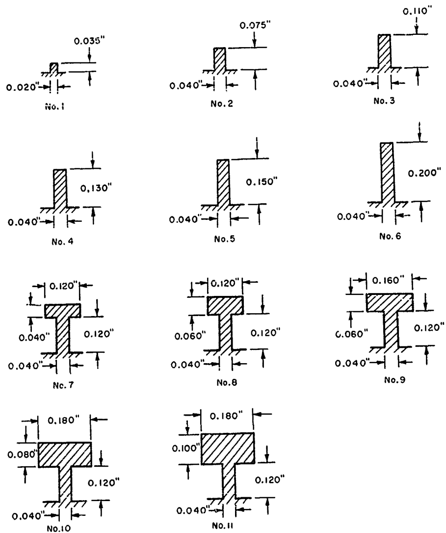
Figure 3 - Heavy-Frame Sections
