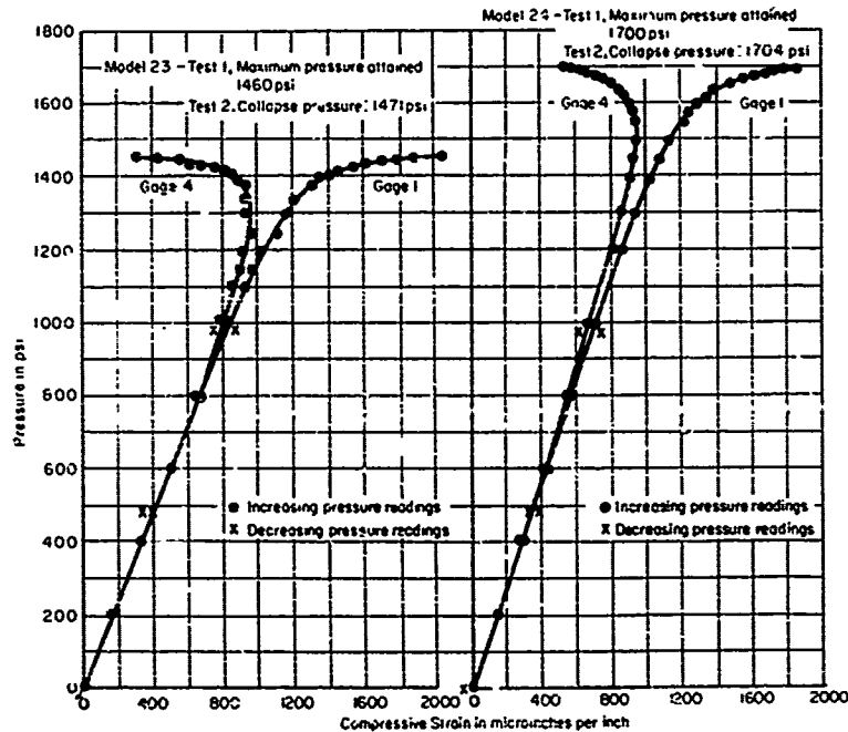
Figure 5 - Representative Experimental Pressure-Strain Plots
