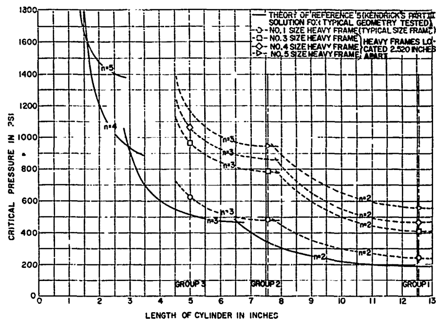
Figure 10 - Theoretical and Experimental Overall Collapse Pressures versus Length of Stiffened Cylinder
