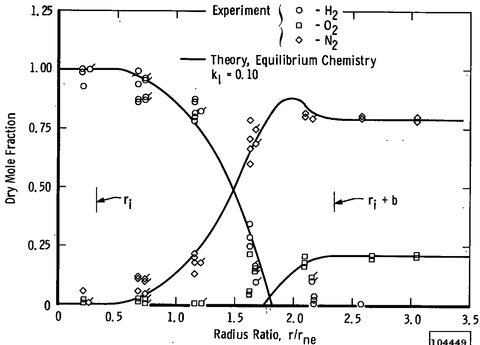
Fig. 17 Radial Composition Distribution at Duct Exit ( O_2 - H_2 Rocket)
