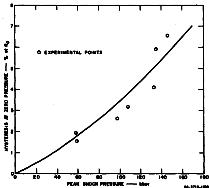
FIG. 9 PRESSURE-RESISTANCE HYSTERESIS OF MANGANIN
