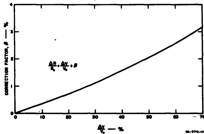
FIG. 22 RECORDING CORRECTION FACTOR \beta , vs. \Delta V/V_0
