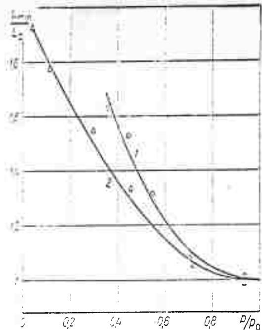
Fig. 22. Dependence of L_{\min} on pressure
