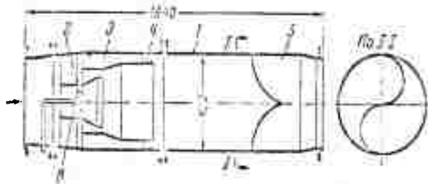
Fig. 25. Diagram of combustion chamber with two-stage swirler for primary air and register for secondary air
