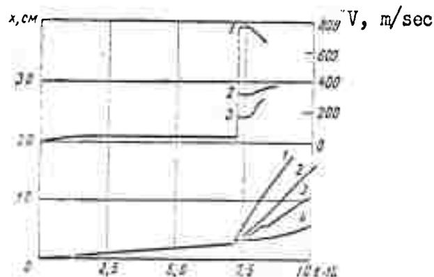
Fig. 6. Time dependence of path travelled by the flame front in hydrogen-oxygen mixtures in a chamber with a diaphragm
