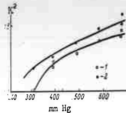
Fig. 2. Dependence of the intensification coefficient K^2 on the initial pressure in the combustion of benzene with nitrogen-oxygen mixtures
