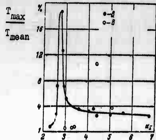
Fig. 31. Low-frequency oscillation amplitudes
