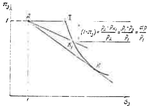
Fig. 17. Deflagration branch of Hugoniot adiabat
