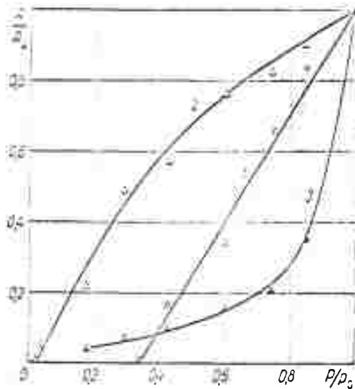
Fig. 20. Amplitudes of flame-front oscillations as a function of pressure
