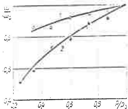
Fig. 21. Effect of pressure on frequency of flame front oscillations
