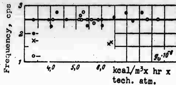
Fig. 30. Dependence of the frequency of low-frequency oscillations on the type of atomizer
