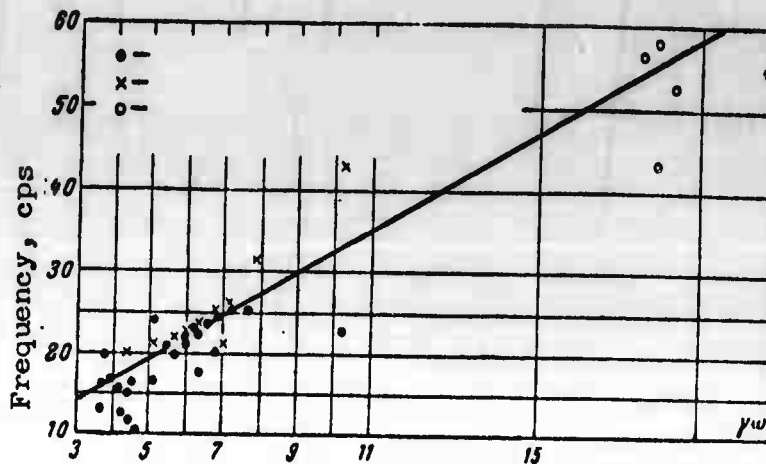
Fig. 28. Dependence of the frequency oscillations on mass velocity of primary air in the combustion region
