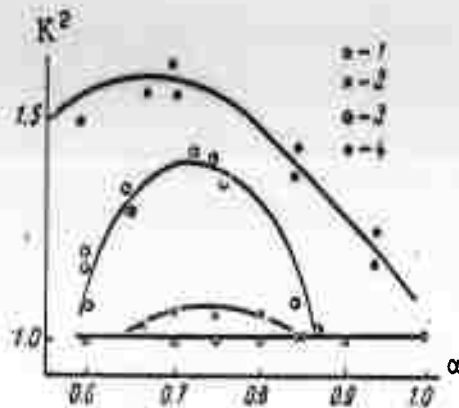
Fig. 1. Dependence of the intensification coefficient K^2 on the mixture composition (air excess factor \alpha ) in the combustion of benzene in nitrogen-oxygen mixtures
