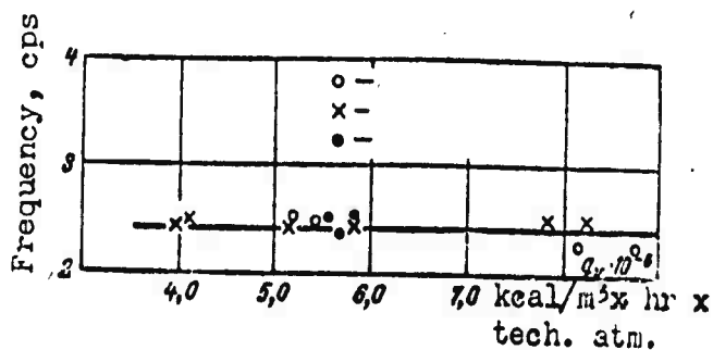
Fig. 29. Dependence of the frequency of low-frequency oscillations on the type of burned fuel
