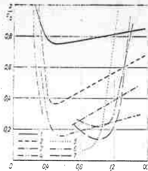
Fig. 19. Limits of oscillatory burning
