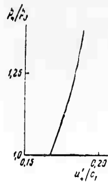
Fig. 14. Dependence of the pressure drop across the shock wave propagating in the products of a steady state deflagration on the dimensionless burning velocity ( u'_1/c_1 ). Calculation by accurate formulas by use of a generalized Hugoniot equation ( \mu = 3 , \gamma = 1.25 , Q/c_1^2 = 30 ).
