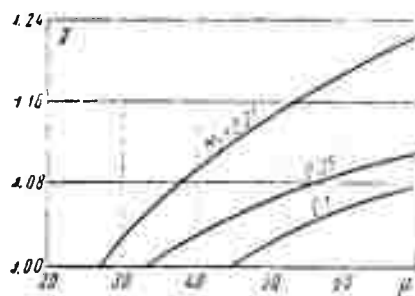
Fig. 18. Stability of one-dimensional gas flow with variable longitudinal temperature gradient
