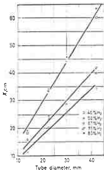
Fig. 4. Dependence of the X value on the diameter of the tube containing the combustible mixture
