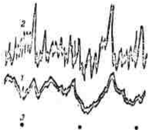
Fig. 26. Oscillograms of temperature and flame-luminosity oscillations
