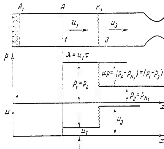
Fig. 16. Diagram of rocket combustion chamber
