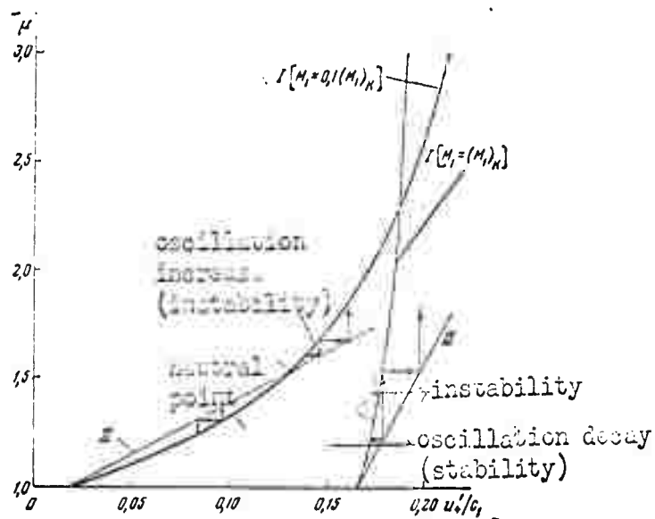
Fig. 15. Dependence of the pressure drop across the shock wave propagating in the fresh gas on the dimensionless burning velocity ( \mu = f(u'_1/c_1) - wave I). These curves were obtained by exact formulas and by use of the generalized Hugoniot equation. Lines II represent the dependence of the dimensionless burning velocity on the pressure drop across the shock wave ( u'_1/c_1 = f(\mu) ). The lines were obtained by analysis of the interaction of weak shock waves with the turbulent combustion zone. Q/c_1^2 = 30 ; \gamma = 2.25 , at M_1 = 0.1 (M_1)_{cr} and M_1 = (M_1)_{cr} .
