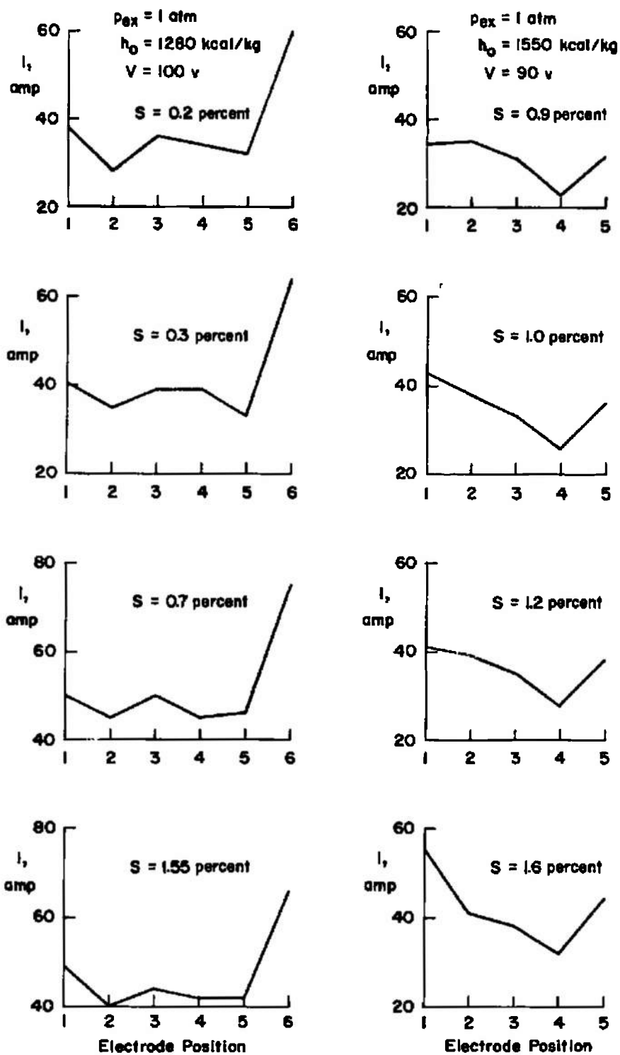
Fig. 24 Effect of Seeding Rate on the Current Distribution in the Axial Direction
