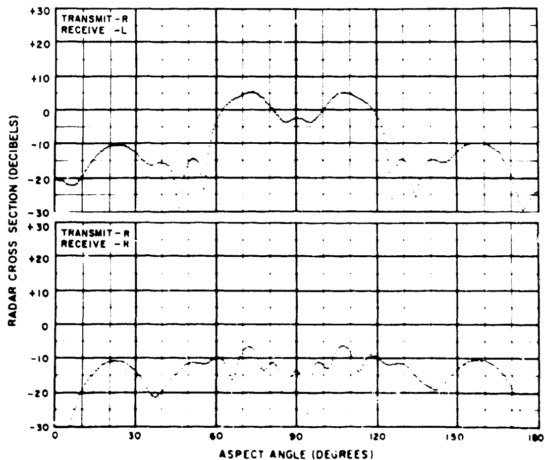
Figure 2-6. Spindly Circular Polarization
