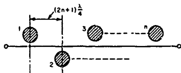
(a) DIELECTRIC RESONATOR BAND STOP FILTER
