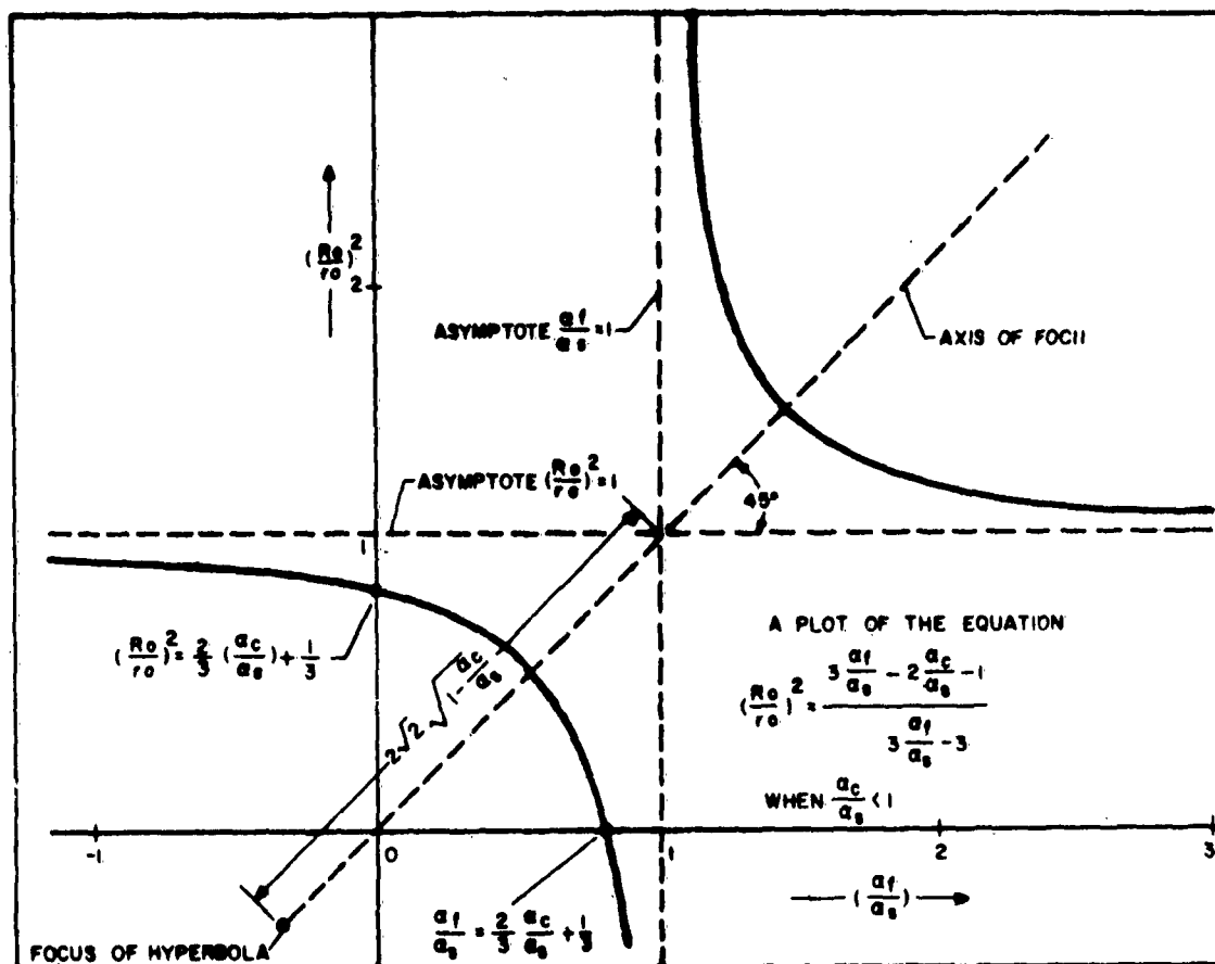
Figure 4-2. Ratio of Radii Versus Filler Expansion Coefficient \alpha_c < \alpha_s
