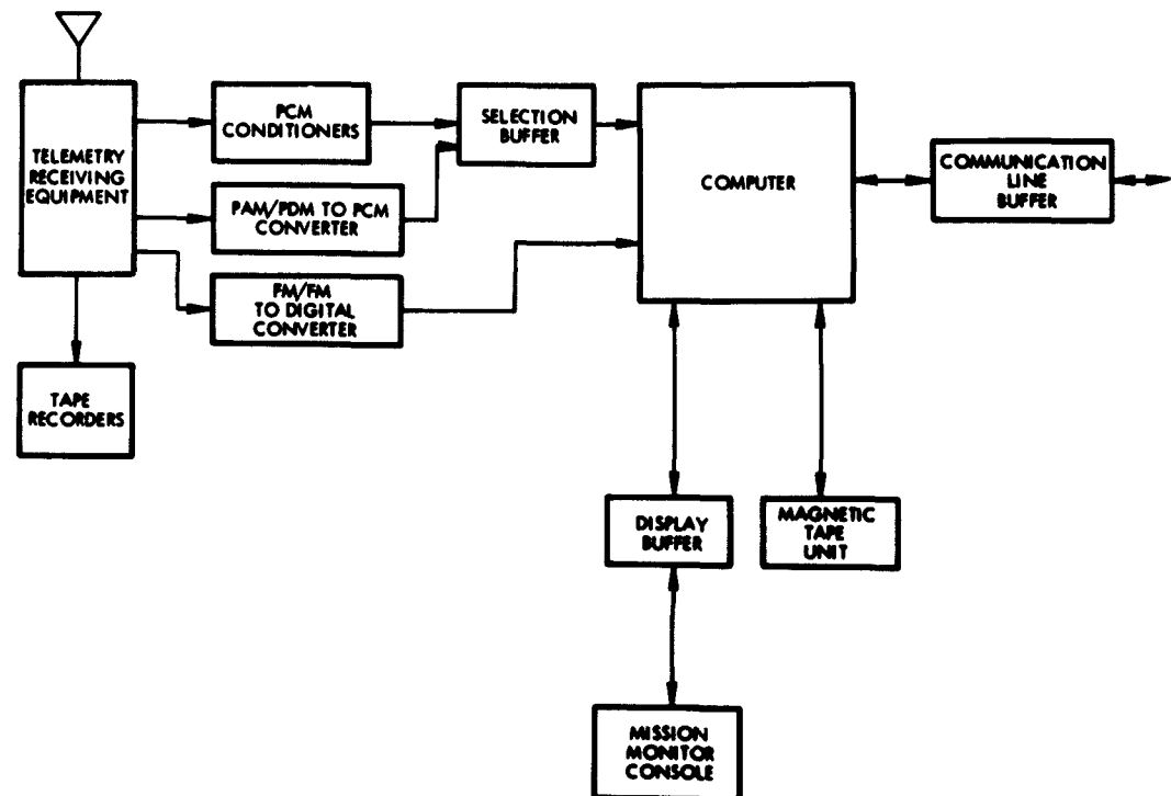
Figure 6. Instrumentation Station Block Diagram
