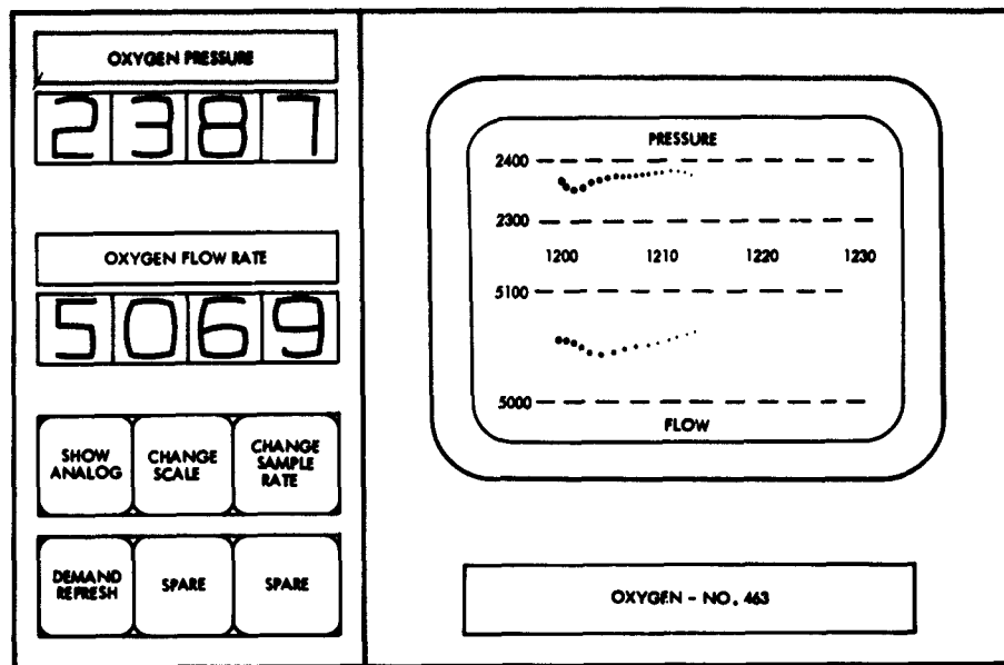
Figure 9. Display Cell
