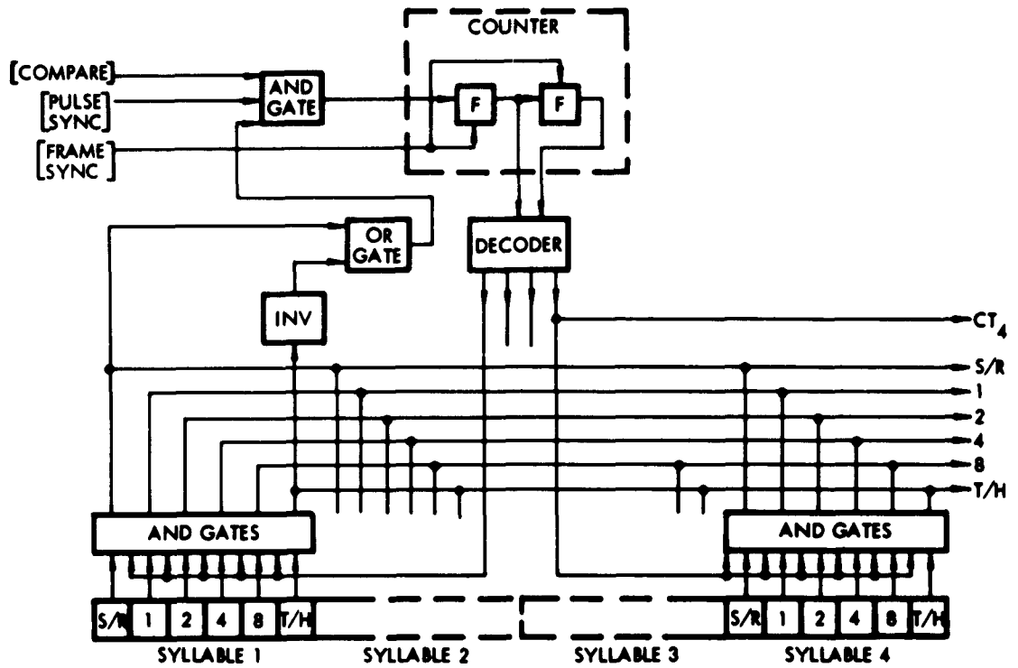
Figure 4. Syllable Multiplexer
