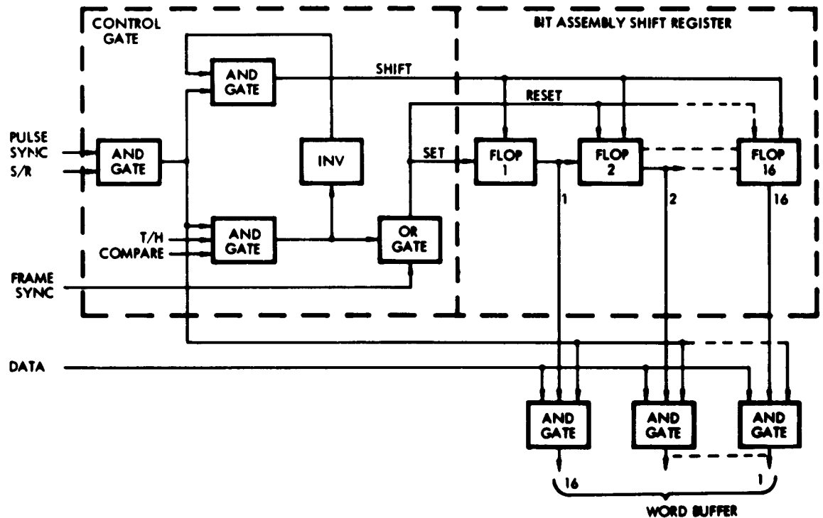
Figure 5. Bit Assembly Shift Register and Controls
