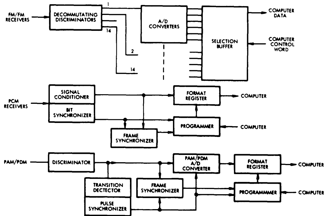
Figure 2. PCM, FM/FM, PAM-PDM System - Simplified Block Diagram
