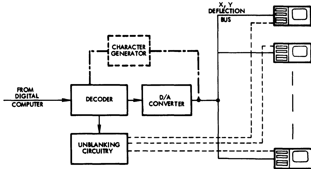
Figure 11. Mission Monitor Console Display Generation and Distribution
