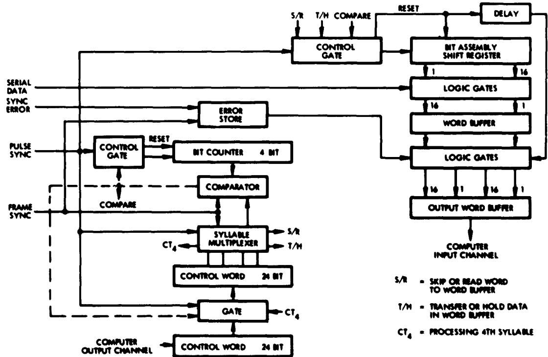
Figure 3. Programmer and Format Register - Simplified Block Diagram
