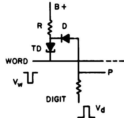
Figure 2. One-Bit Memory Cell
