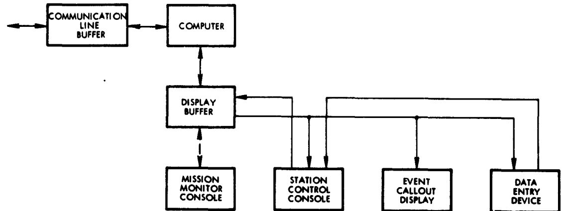
Figure 12. Instrumentation Station Control System
