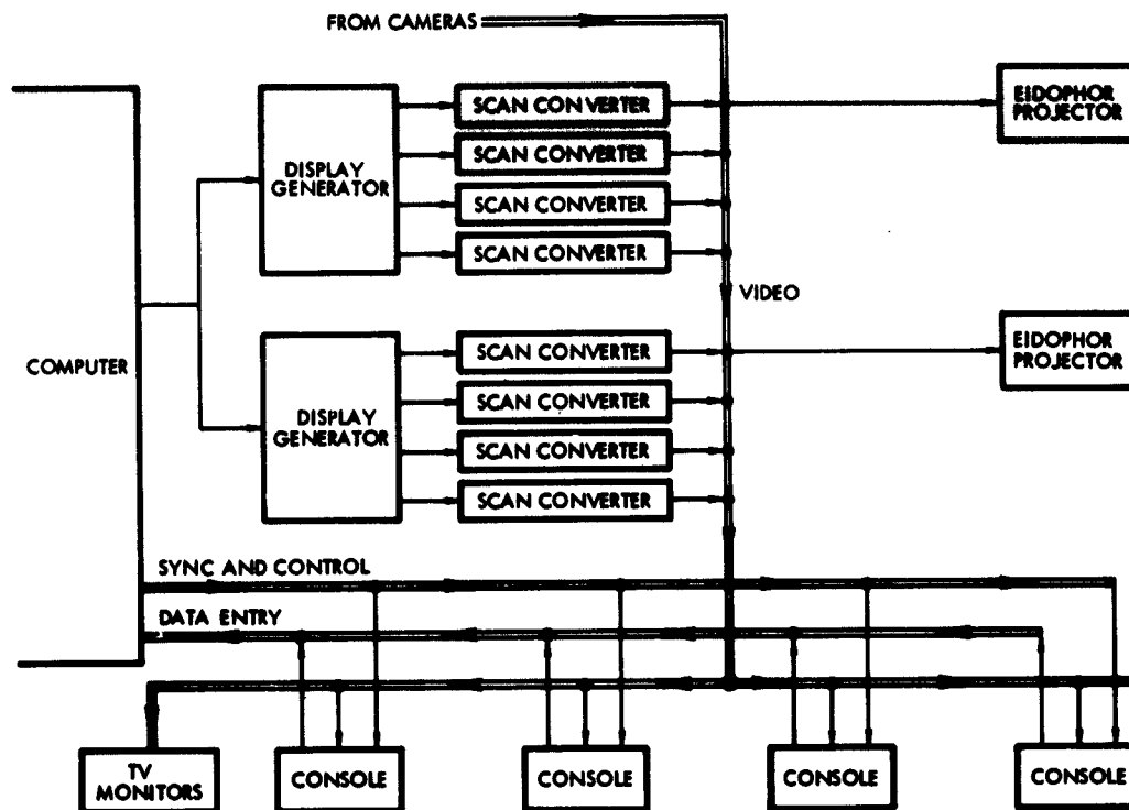
Figure 7. Display Generation and Distribution System
