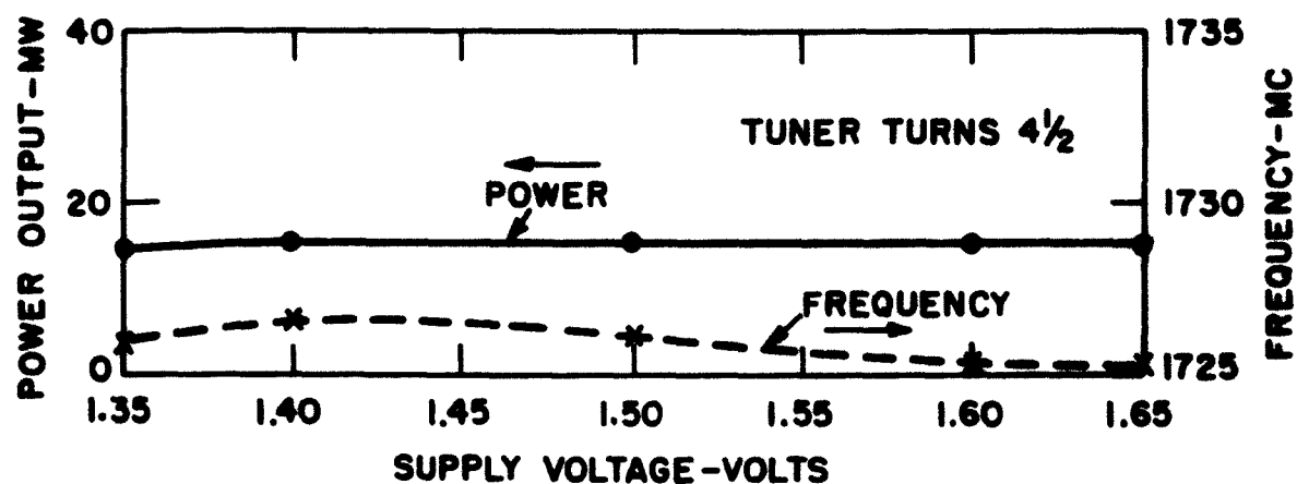
FIG.38 POWER OUTPUT AND FREQUENCY TUNNEL DIODE OSCILLATOR S-II6 SERIAL 006.
