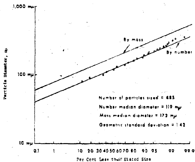
Figure 3. Size Distribution of Radioactive T1 Phage Aerosol at 55% Relative Humidity Dispersed with Bantrolane D 30 Aerosol Generator.
