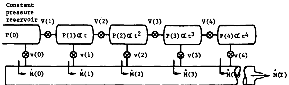
Figure 2. An idealized fourth-degree polynomial gas mass flow rate system. The areas labeled with P(n) are the tanks which receive gas through valves, V(n) , on the left and discharge gas to the succeeding tank through valves, V(n+1) , on the right and to the plenum below through valves, v(n) . All valves are vernier controlled sonic throttles. The system is assumed to be isothermal although a real system built on this principle may not be isothermal and will require compensating adjustments of the valves.
