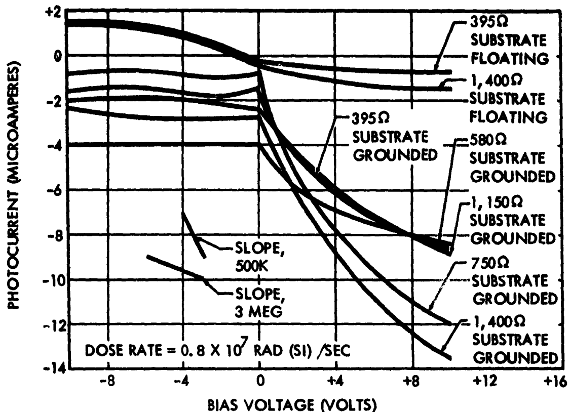
Figure 5. Photocurrent versus bias voltage for Fairchild resistors \mu\text{ER-1} .
