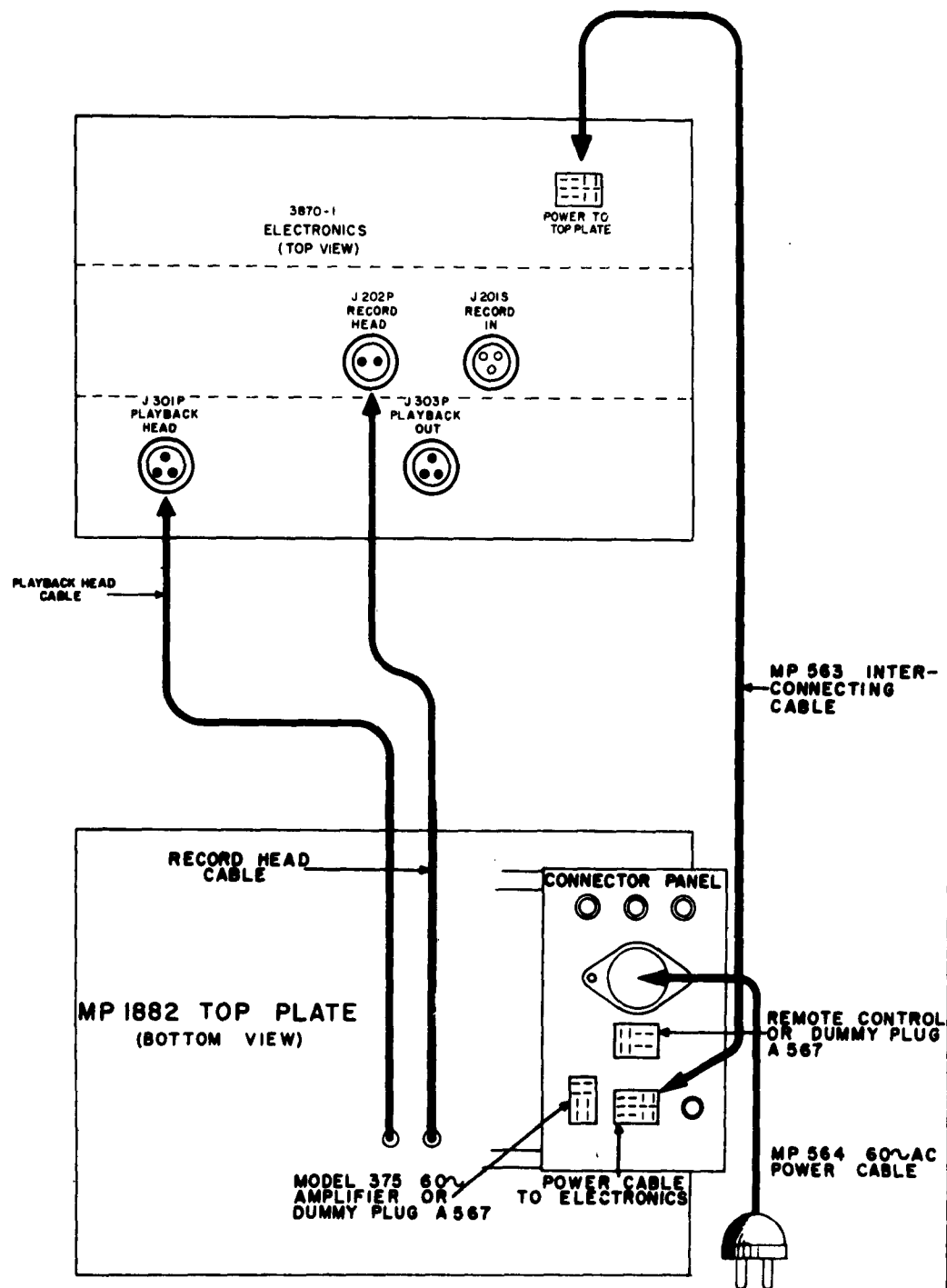
INTER UNIT CONNECTION DIAGRAM MODEL 306-I
