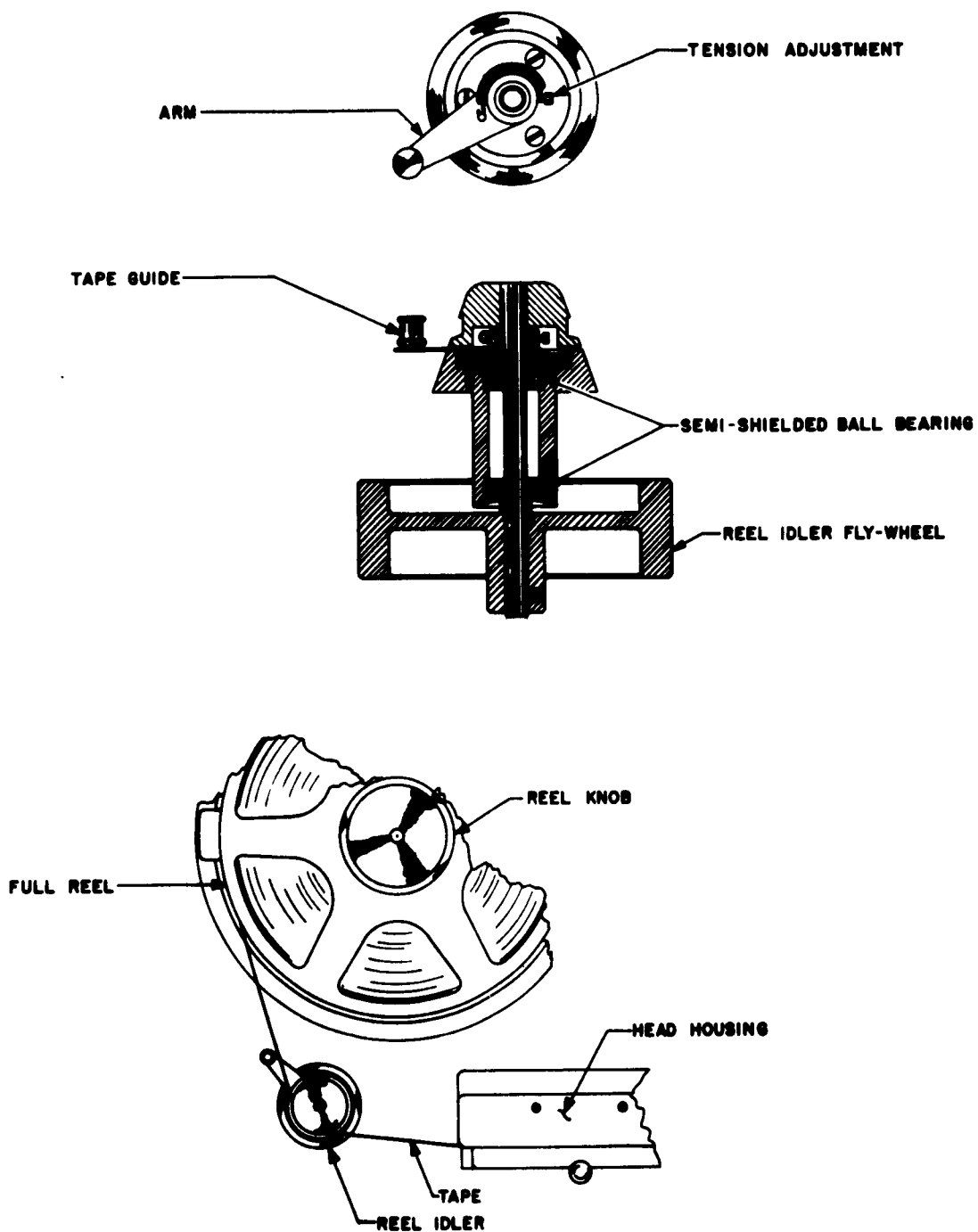
REEL IDLER ASSEMBLY SERIES 300 AMPEX ELECTRIC CORPORATION REDWOOD CITY, CALIFORNIA
