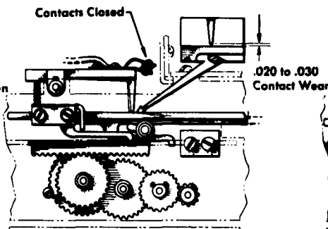
TIMING POSITION (Contacts Closed)
