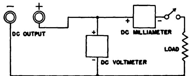
RAPID CHECK SETUP
