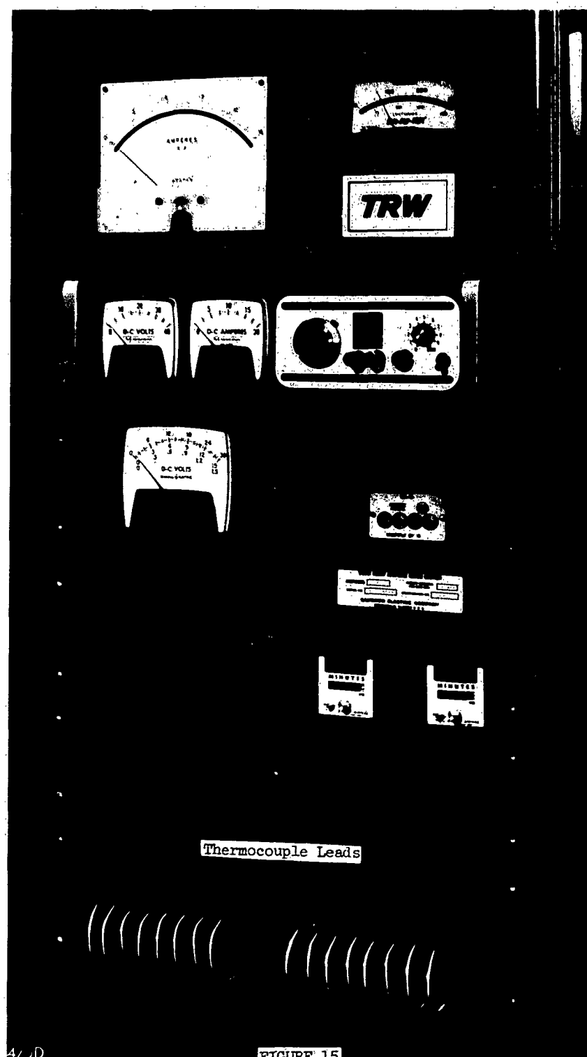
4/ J.D. FIGURE 15 ELECTRICAL INSTRUMENTATION PANEL
