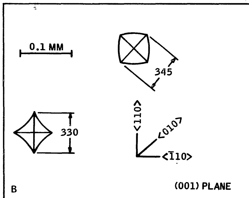
FIGURE 3. ANISOTROPY OF VICKERS HARDNESS ON THE (110) AND (001) PLANES IN AN ANNEALED CRYSTAL
