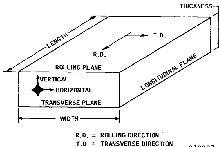
FIGURE 1. FACES AND RELATED DIRECTIONS OF ROLLED SINGLE CRYSTAL BILLET
