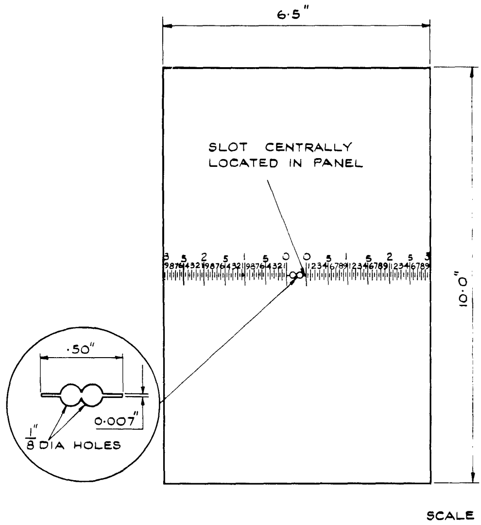
CRACK PROPAGATION PANEL
