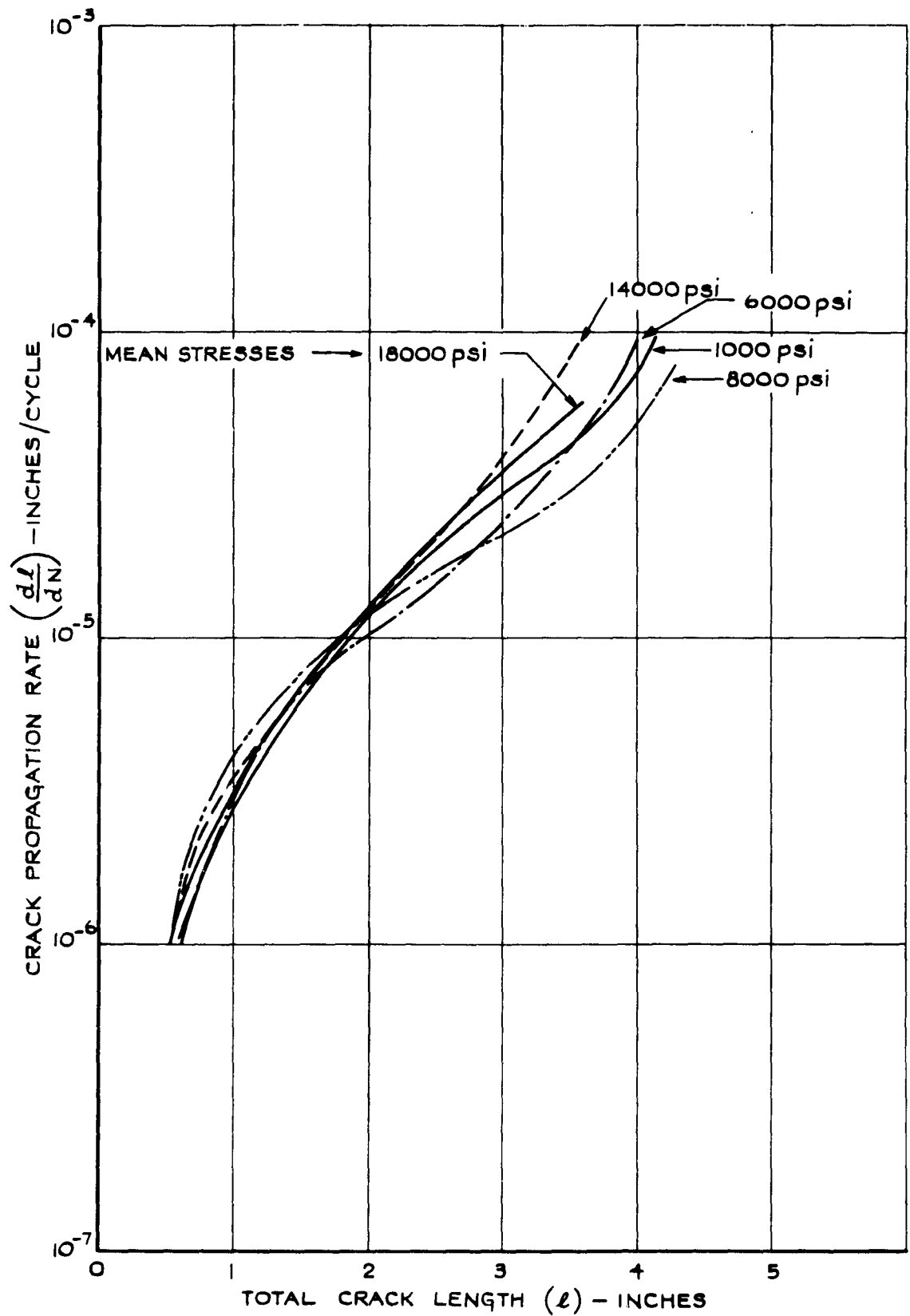
FIG.18 EFFECT OF MEAN STRESS ON CRACK PROPAGATION RATES IN D.T.D 546B SHEET (ALTERNATING STRESS \pm 2000 psi IN ALL TESTS)
