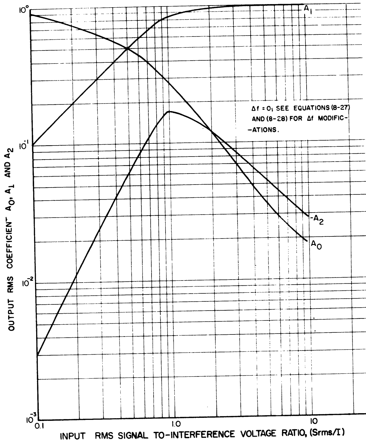
Figure 8-2. Normalized Carrier Amplitudes for Output Interference Due to Interaction of Input Pulse Interference with Desired Signal [\overline{m_s^2(t)} \leq 0.1]
