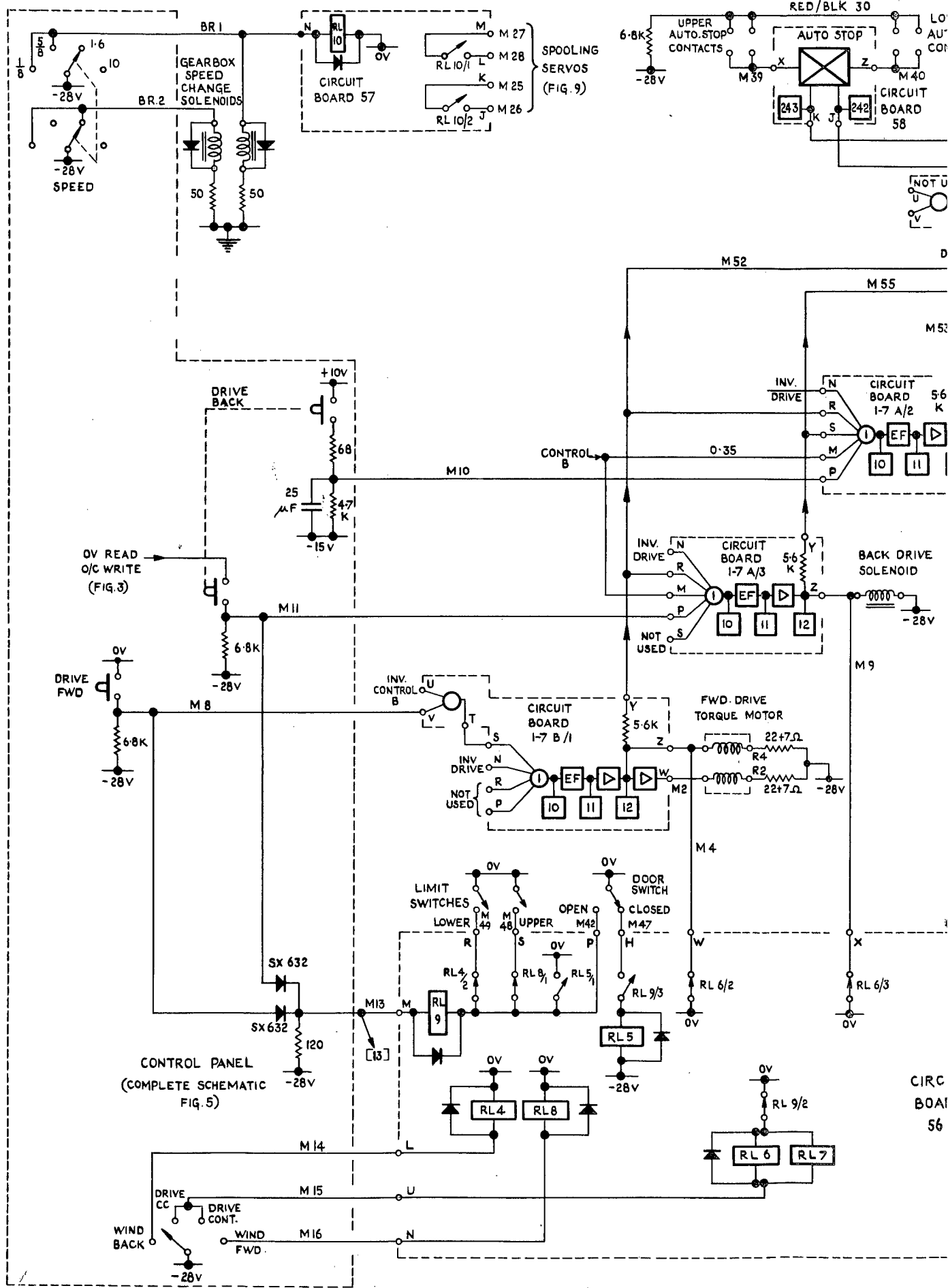
FIG. 7 TAPE DRIVE AND TAPE V
