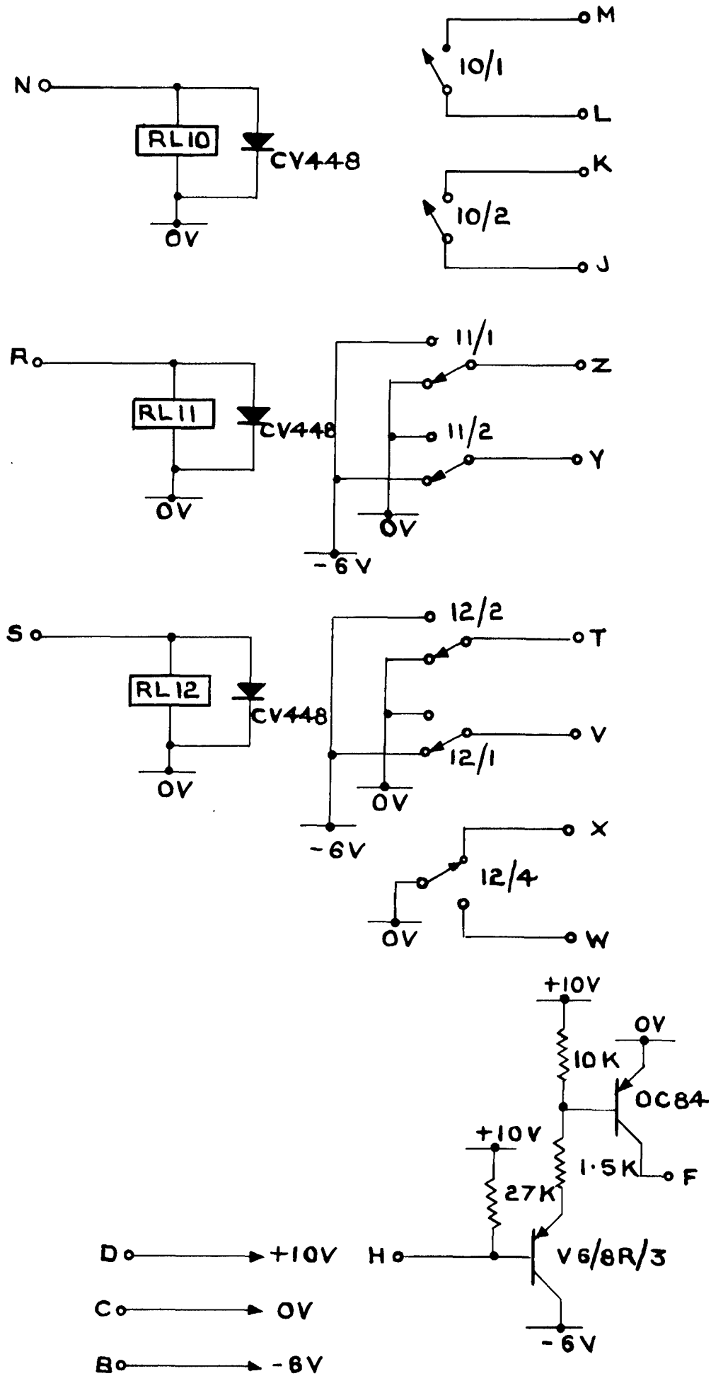
FIG. 22 CIRCUIT BOARD 57 (FUNCTION RELAYS)
