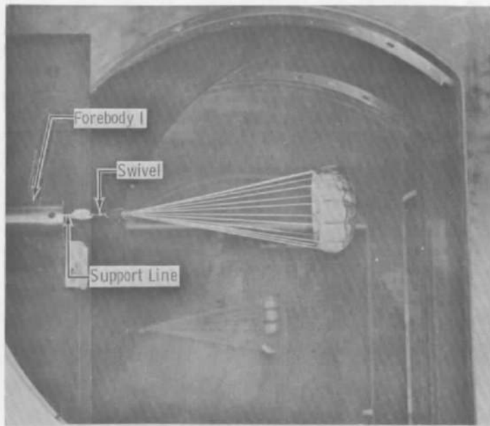
Hyperflo Configuration 2, M_\infty = 3
