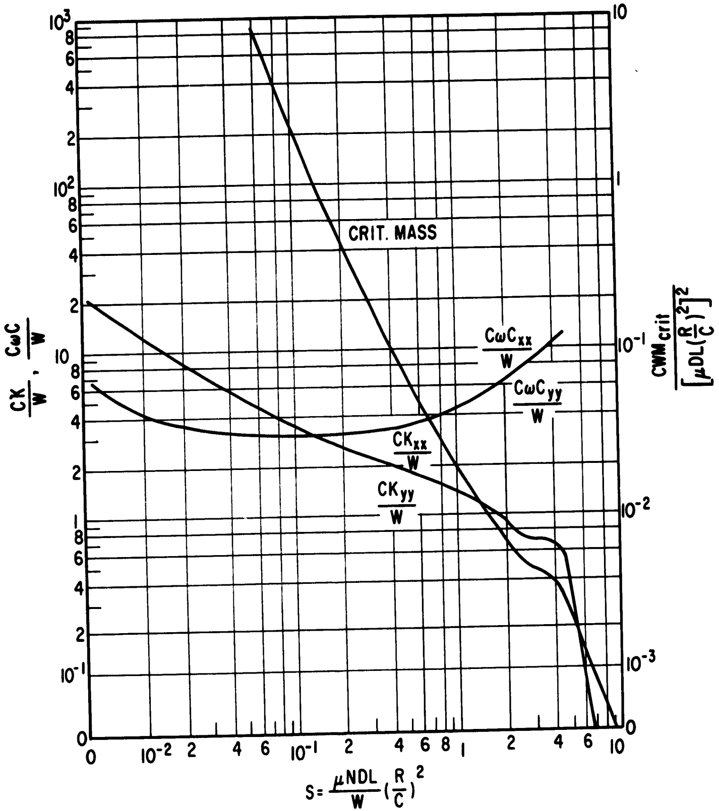
Fig. 8 Four 80° Tilting Pads, Centrally pivoted, L/D = .75 , L/B = 1.074 , C'/C = 1 . Load between pads. No pad inertia.
