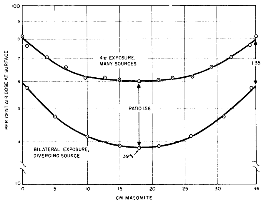
DEPTH DOSE DISTRIBUTION IN CYLINDRICAL PHANTOM, CO 60 FACILITY, (NMRI)
