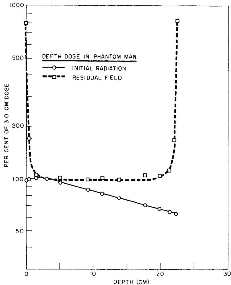
Fig. 1.5 Comparative Depth Doses in a Phantom Man of Initial Atomic Bomb Radiation and Radiation from a Field of Fission Products
