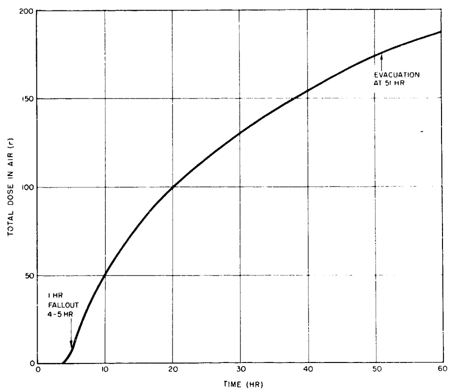
Fig. 1.3 Cumulative Dose as a Function of Time After the Detonation
