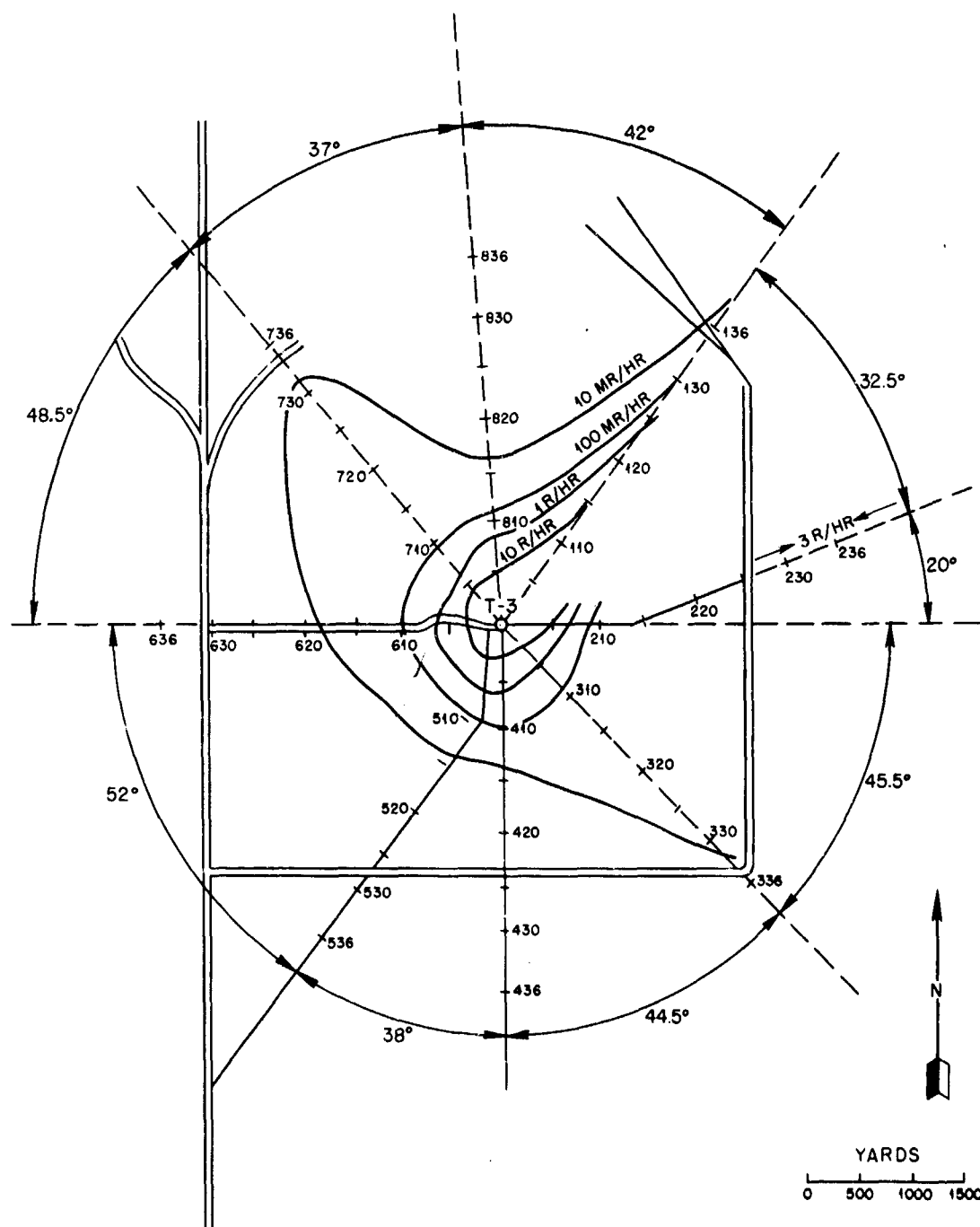
Fig. 3.6—Initial survey, Moth. Area, T-3; date, 22 February 1955; survey time, 0612 to 0730 hr.
