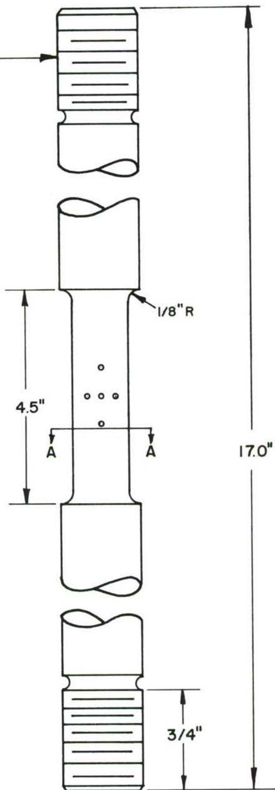
FIGURE 37-MACHINED INCONEL X-750 TEST SPECIMEN
