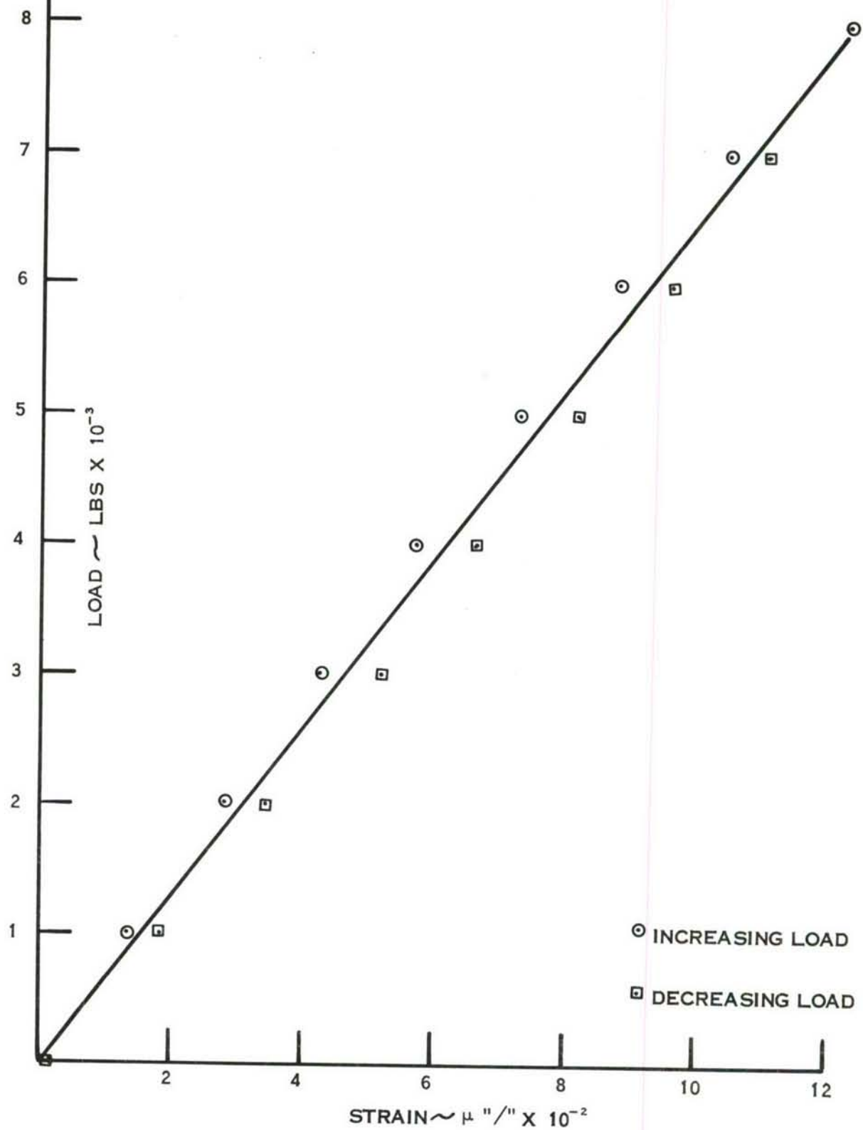
FIGURE 28 STRAIN SENSITIVITY OF AN OPTICAL GAGE AFTER EXPOSURE TO 1200°F AT 75°F ON NICKEL
