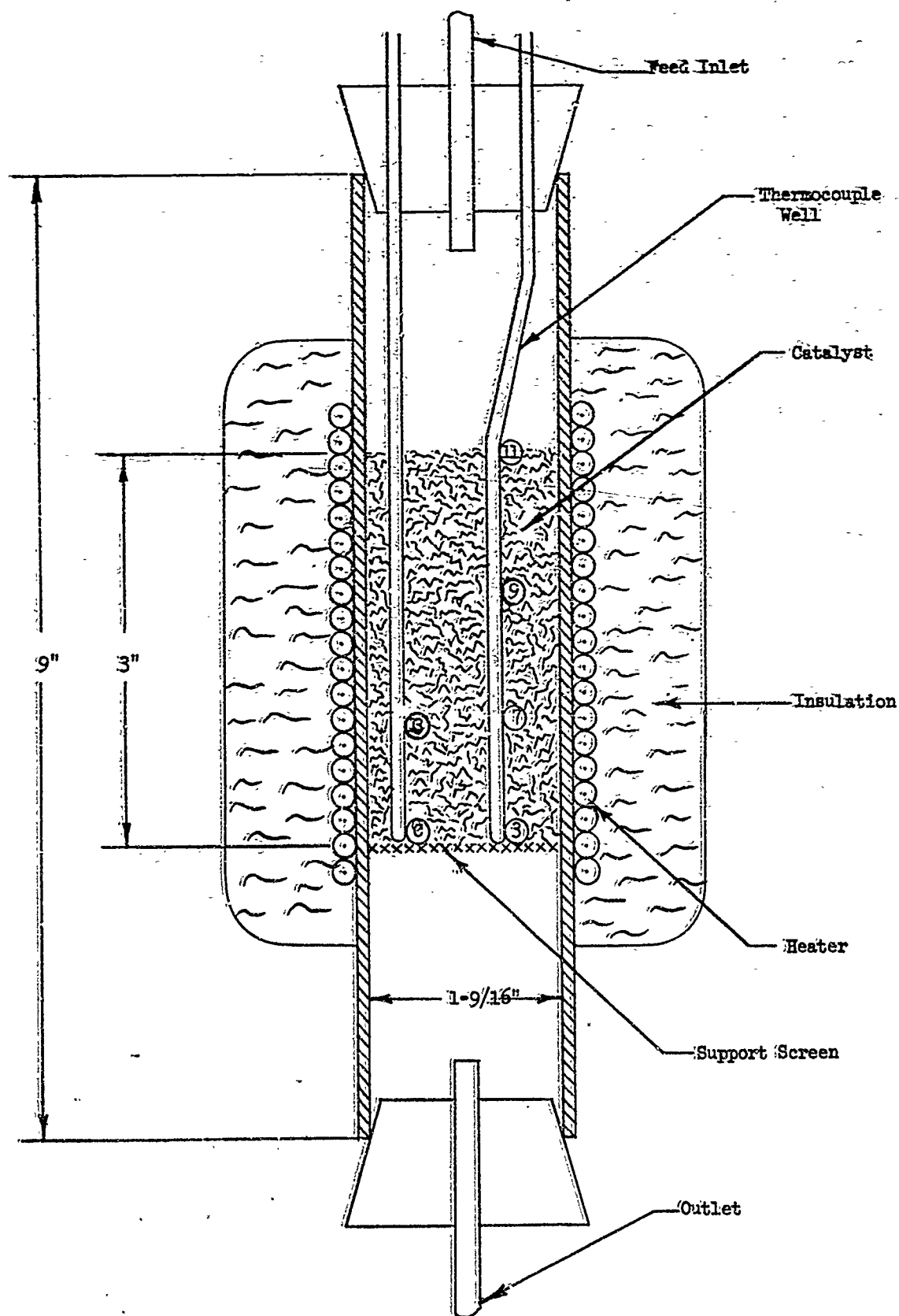
Figure 3 2-G REACTOR SCHEMATIC DRAWING
