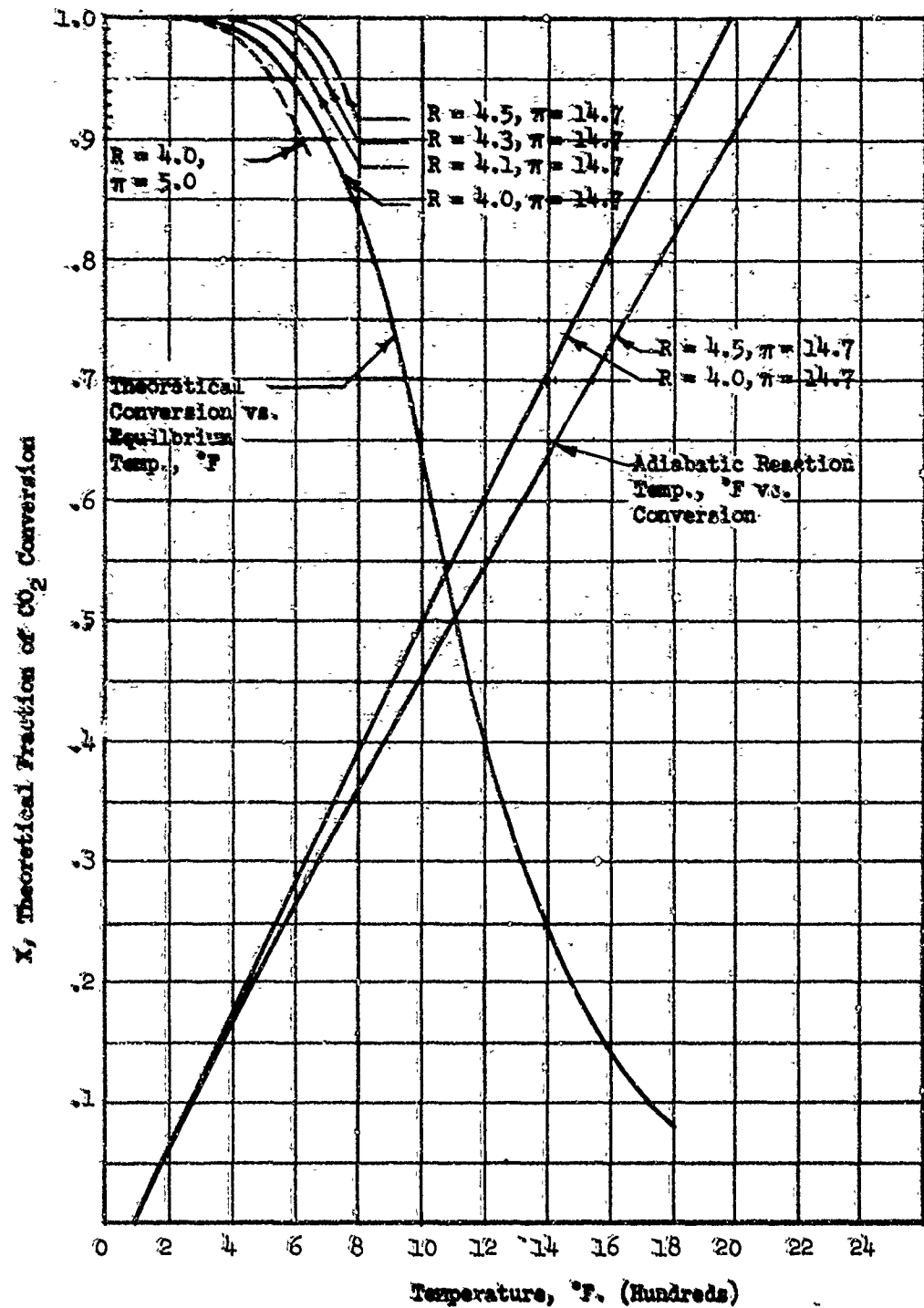
Figure 7 THEORETICAL \text{CO}_2 EQUILIBRIUM CONVERSION VS. TEMPERATURE
