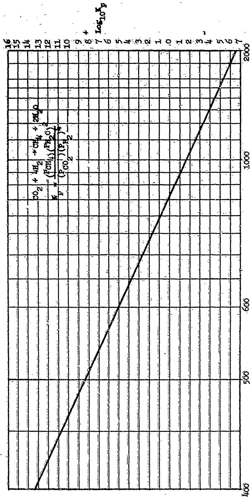
Reaction Temperature, °K. Figure 6 EQUILIBRIUM CONSTANT VS. TEMPERATURE
