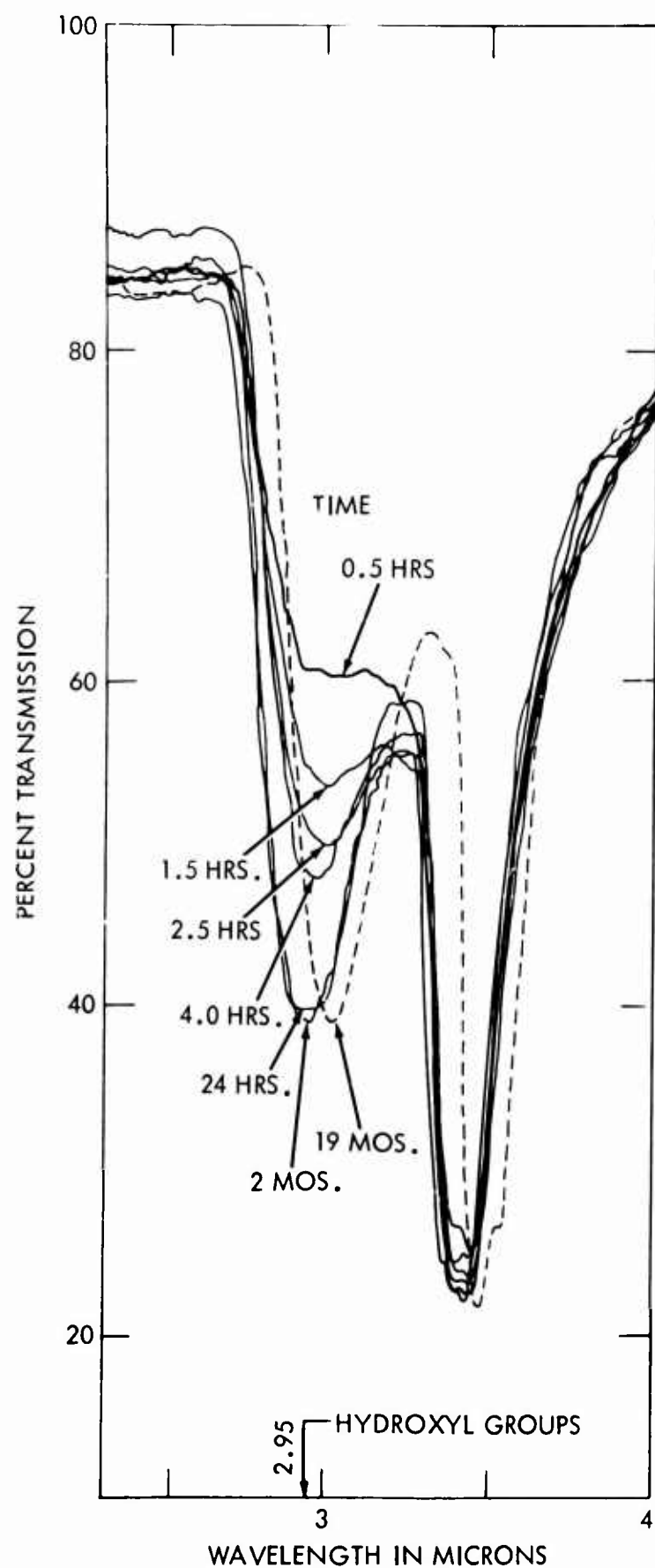
FIG. 7 SPECTRA DURING POLYMERIZATION OF CASTAPLAST 247, CURED AND STORED AT ROOM TEMPERATURE
