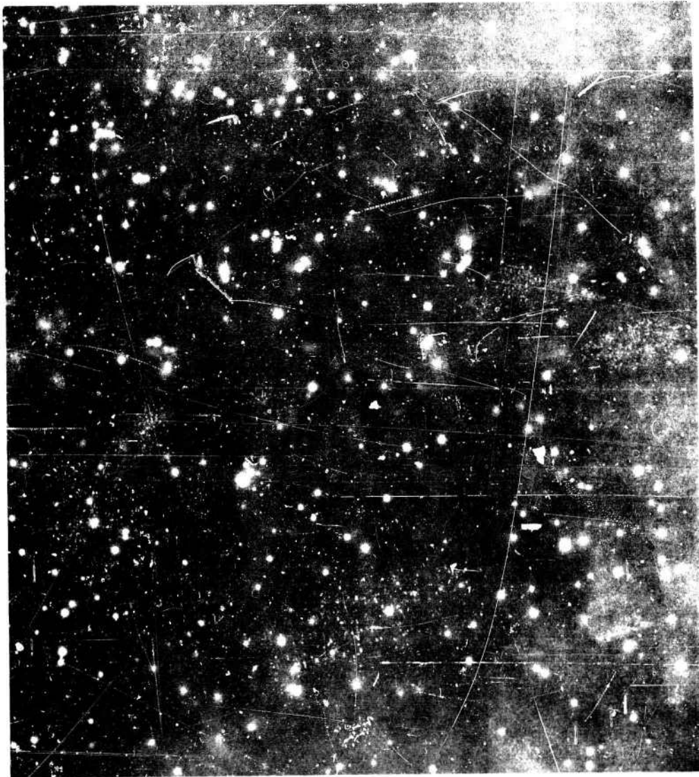
Fig. 5.1—Radioautograph of secondary fall-out particles.
