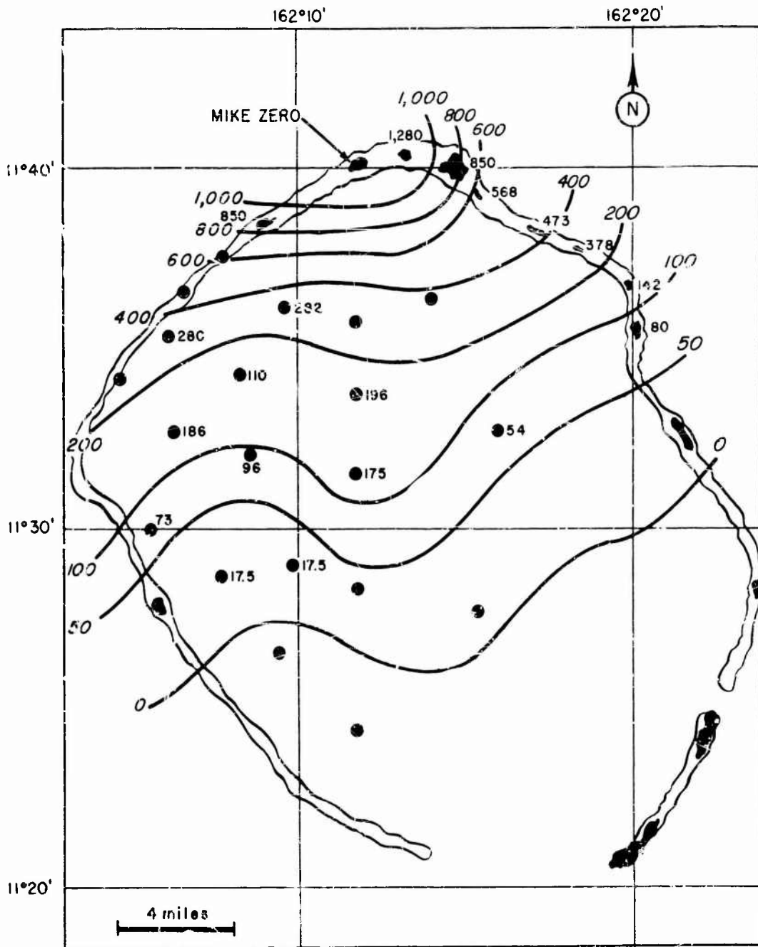
Fig. 4.1—Fall-out gamma pattern at 2 hr as would be experienced on a land mass (t/hr).
