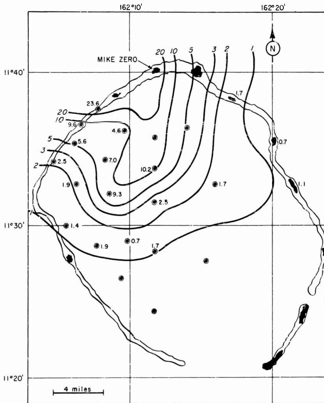
Fig. 4.8—Mass distribution of fall-out (g/sq ft).
