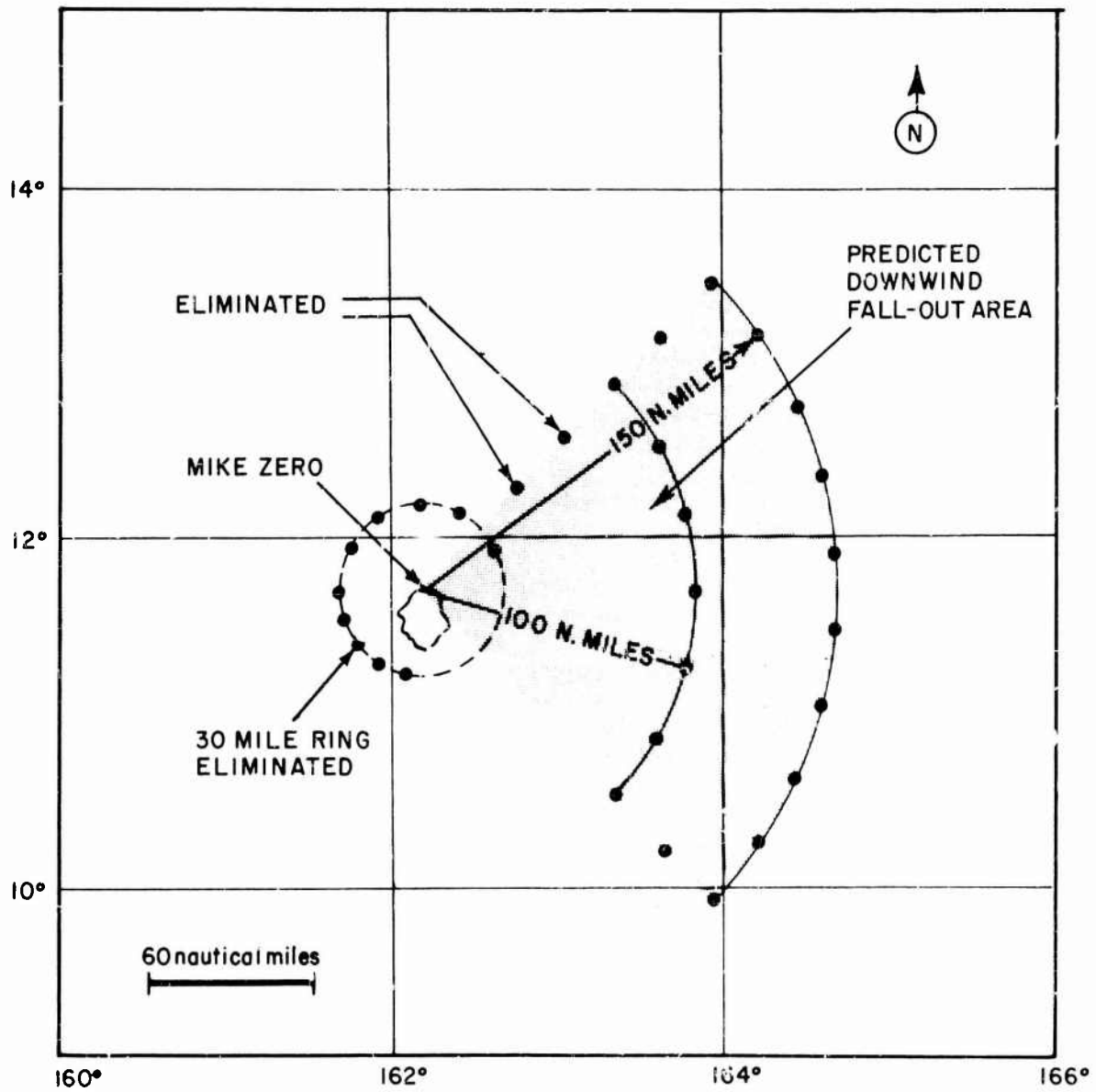
Fig. 2.3—Free-floating sea-station array.
