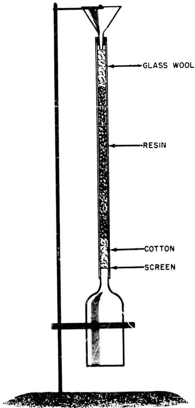
Fig. 3.8—Ion-exchange-column collector.
