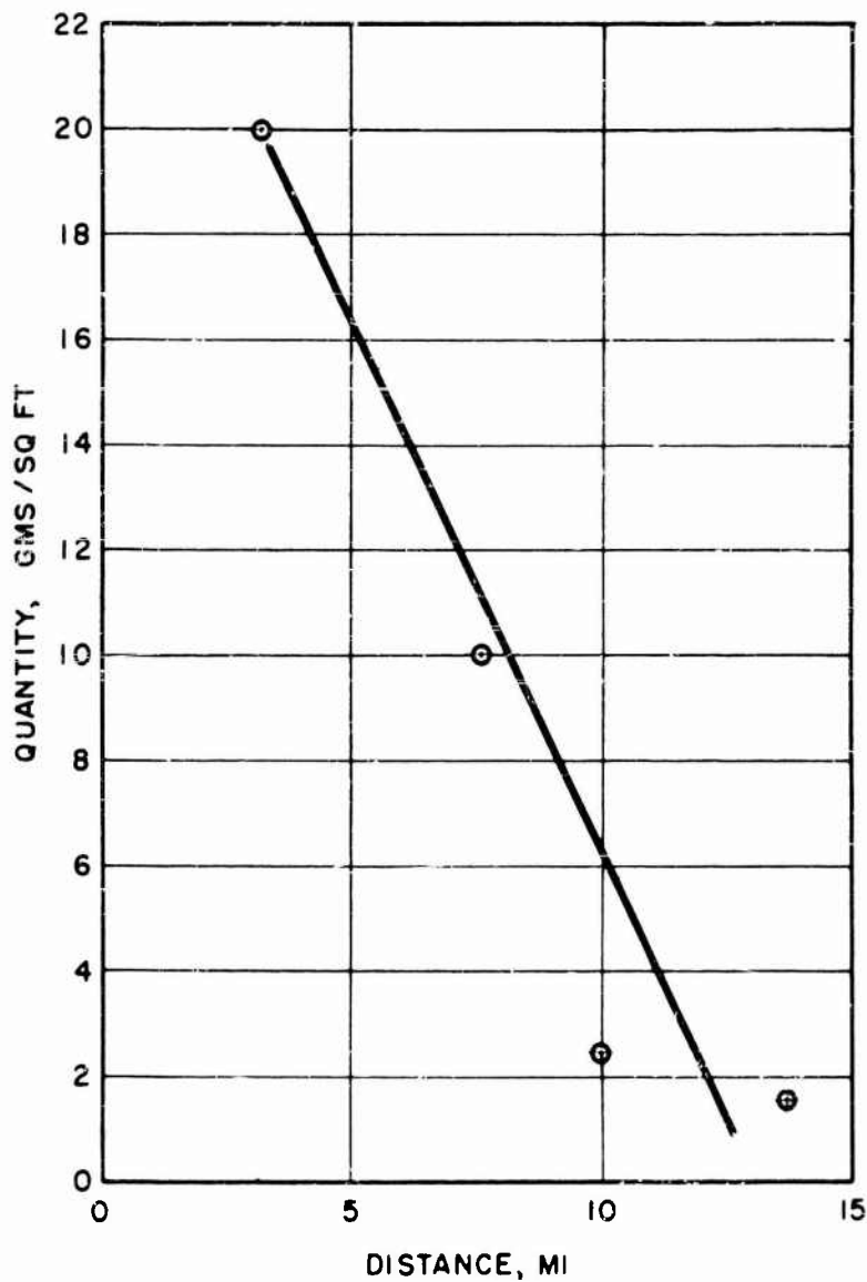
Fig. 4.9—Variation of cross-wind fall-out with distance from ground zero.
