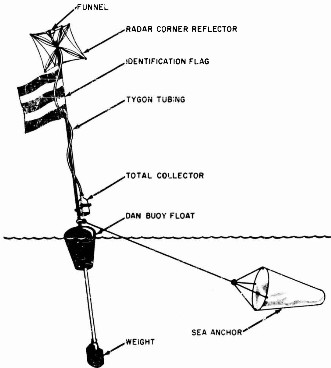
Fig. 3.10—Free-floating sea station.
