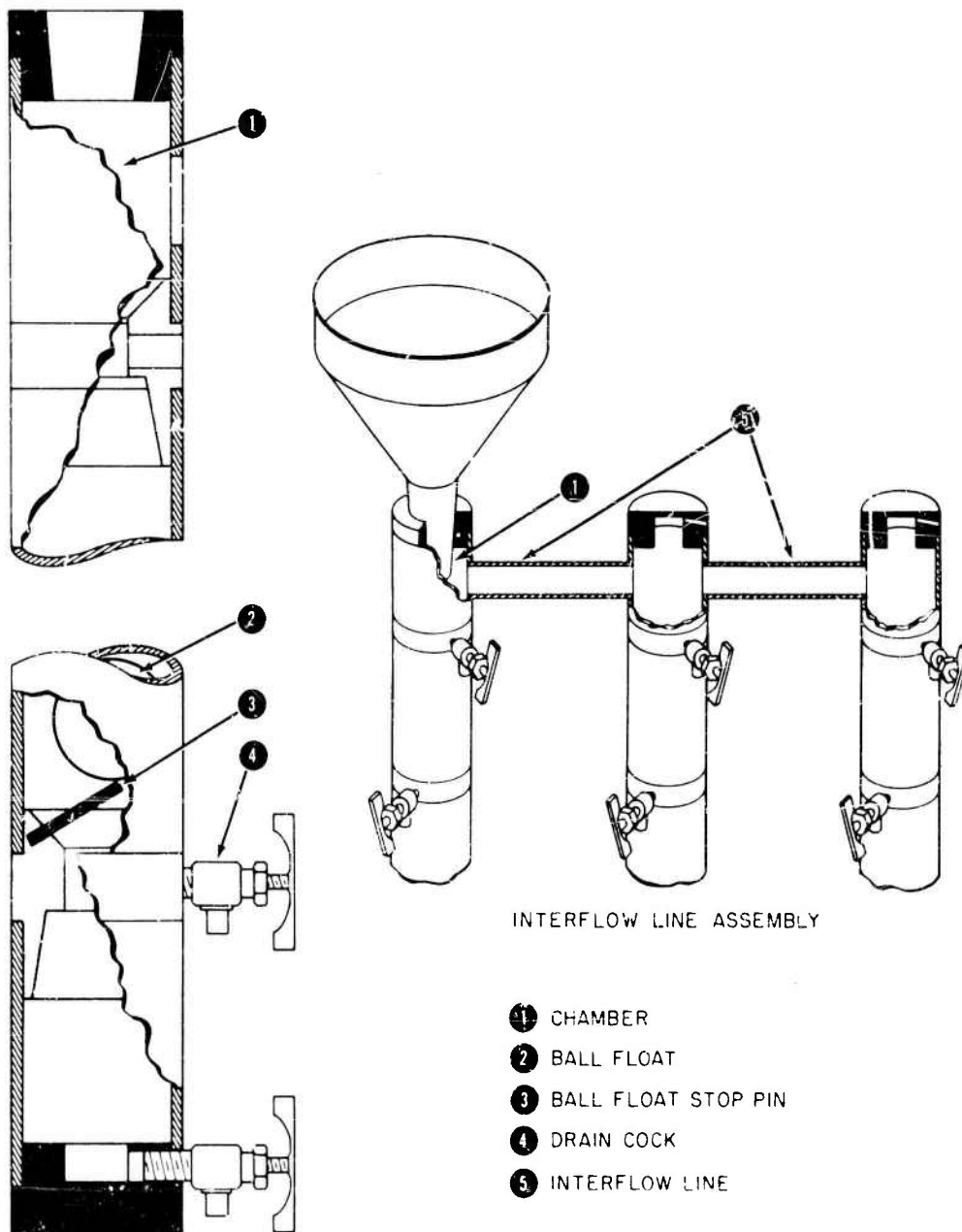
Fig. 3.4—Incremental liquid fall-out collector.
