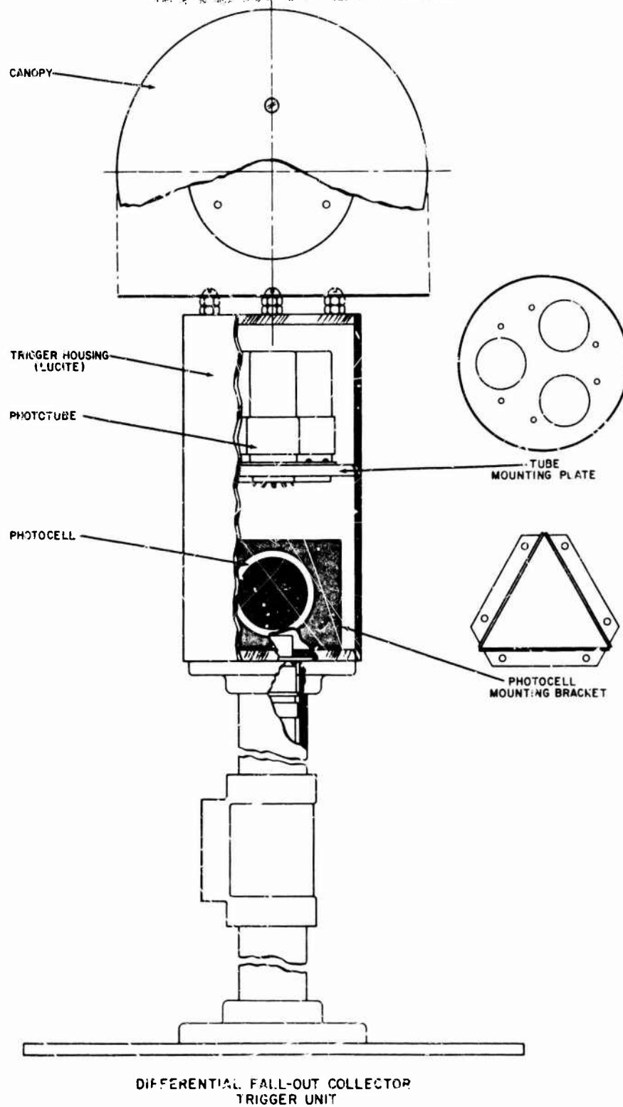
Fig. 3.3—Light-actuated trigger mechanism.
