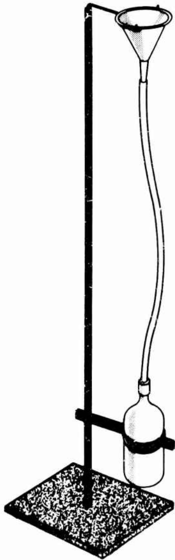
Fig. 3.1 — Total fall-out collector.
