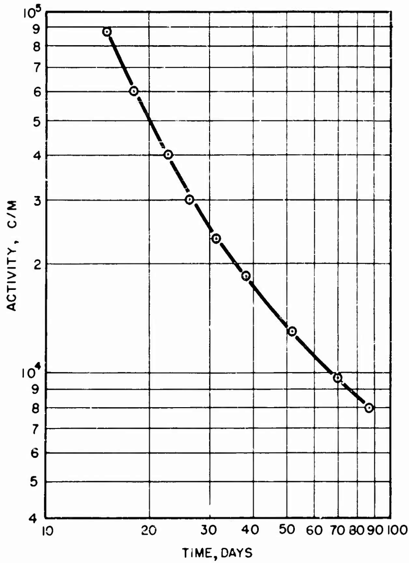
Fig. 4.7—Beta and gamma decay curve from 15 to 90 days after shot.
