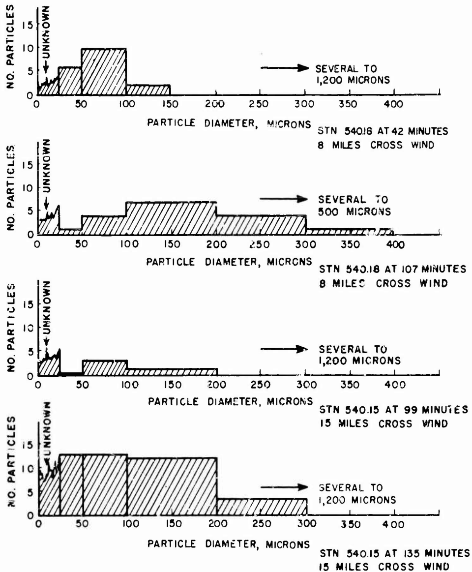
Fig. 4.10—Size distribution of radioactive particles as a function of time and distance.
