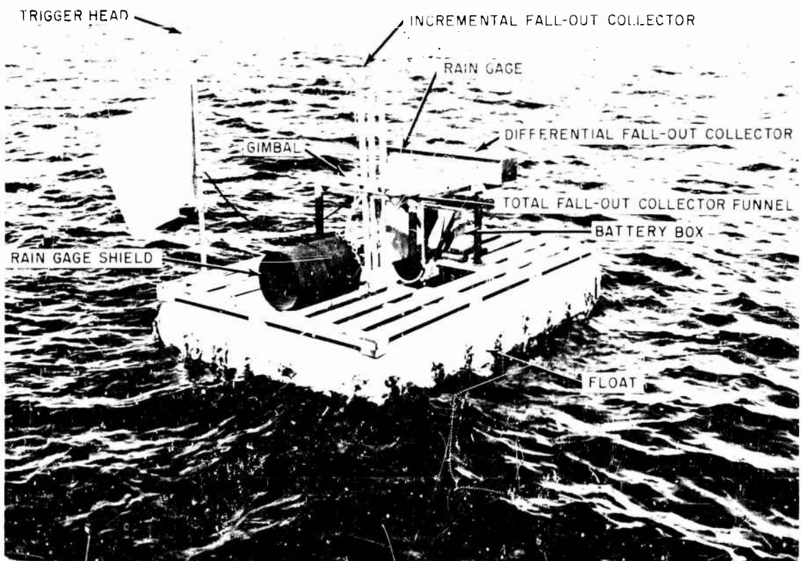
Fig. 3.9—A typical lagoon station.
