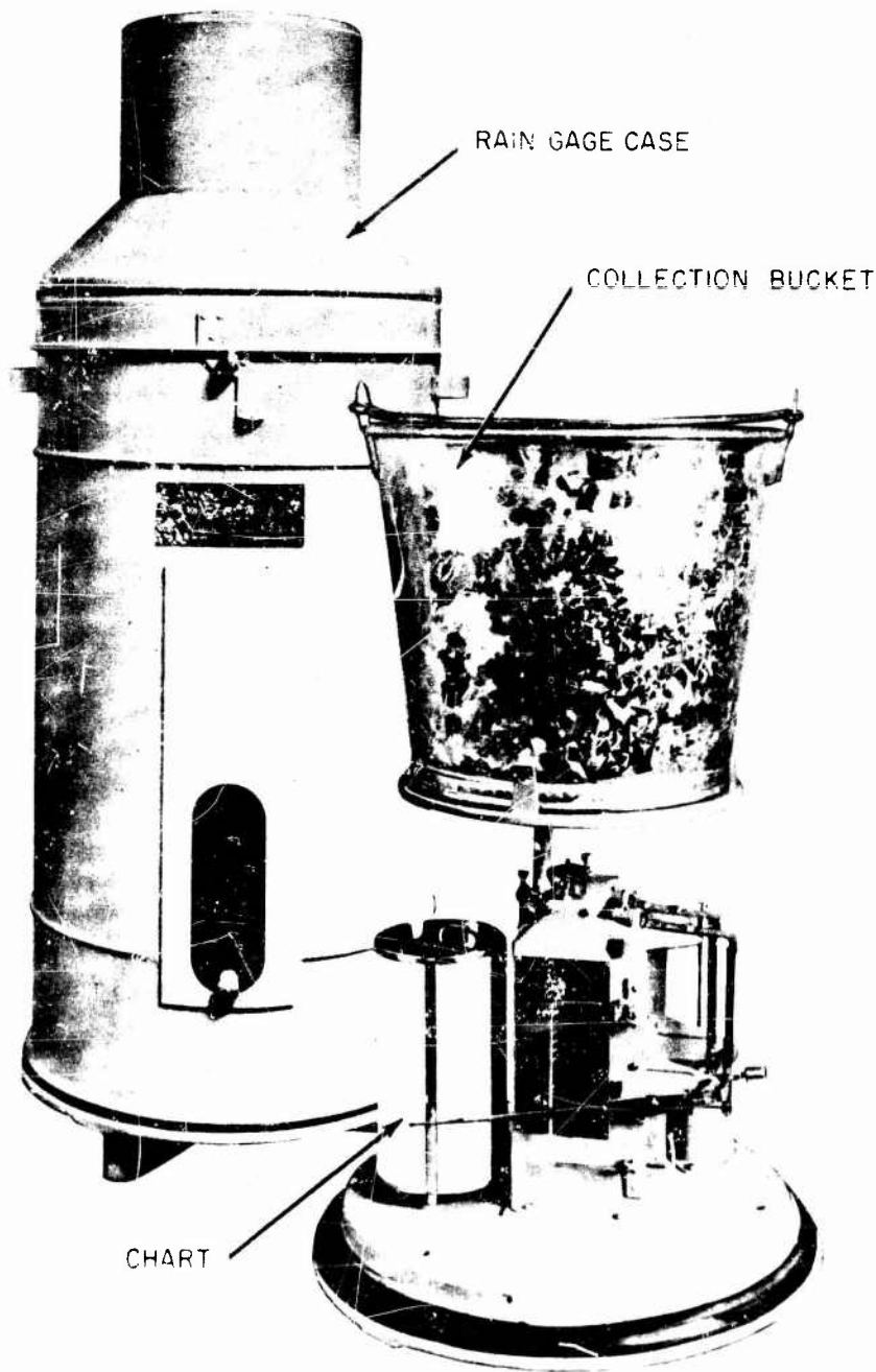
Fig. 3.5—Recording rain gage.
