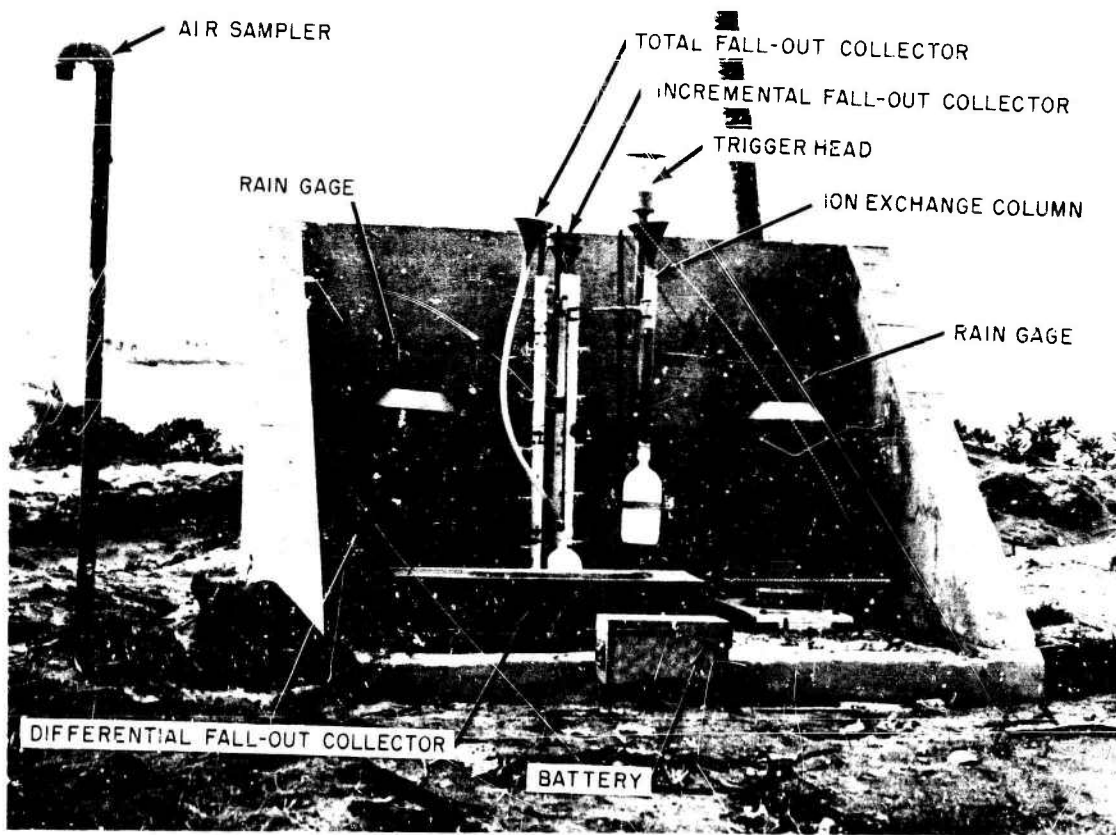
Fig. 3.8—A typical land station.
